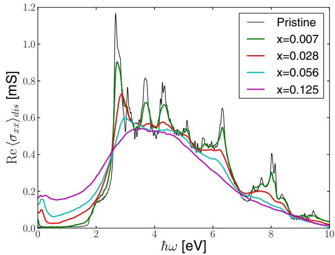
FIG. 7. (Color online) Configuration-averaged optical absorption spectrum of MoS 2 at various impurity concentration.
