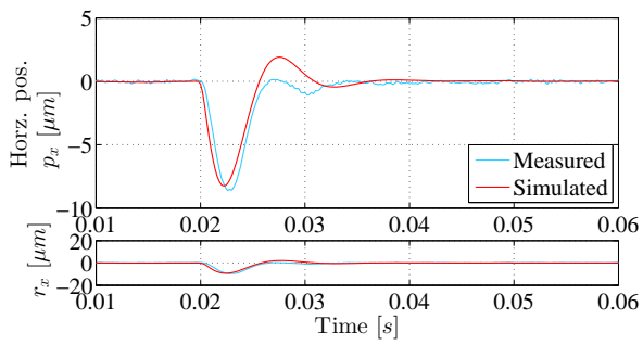
Figure 24: Simulated and measured horizontal closed loop impact response.
