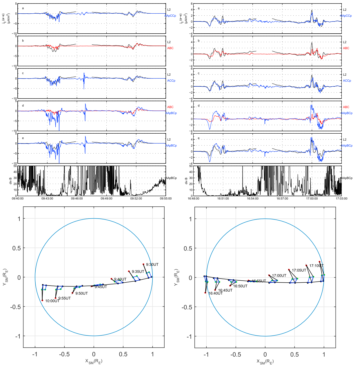
Figure 3. Set of curlometer comparisons in the same format as Figure 2, with the X-Y SM projections of the configurations, including time-shifted positions, shown in the bottom plots. The left-hand plots correspond to the pass on the 28 April 2014 and the right-hand plot to the 4 May 2014.
