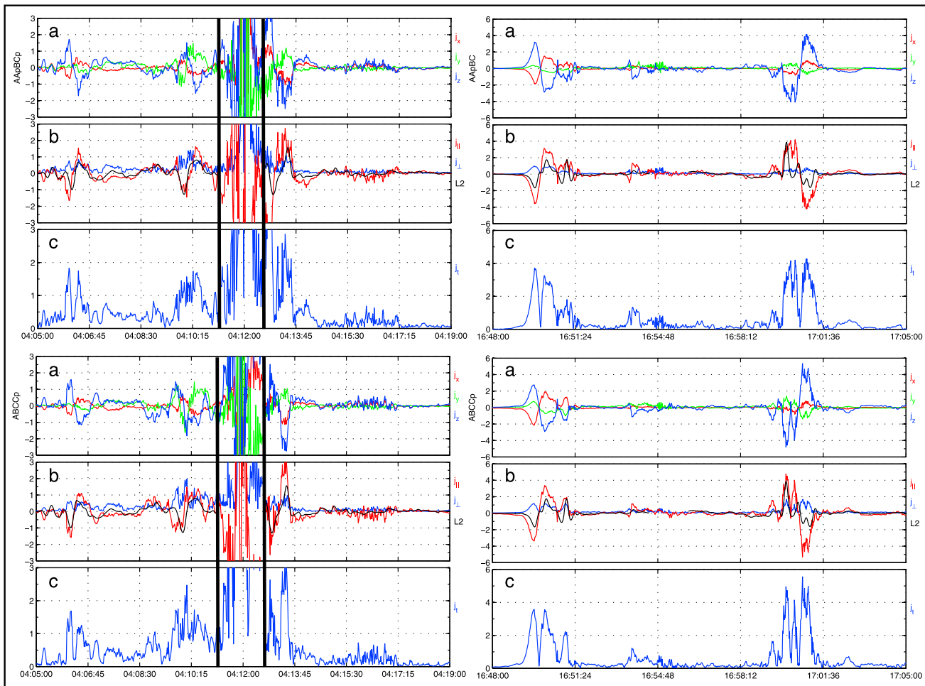
Figure 4. Vector current density estimates obtained from the 4-point estimates for the key intervals during the 22 April (left) and 4 May (right) passes. For each event we plot the estimates from two configuration choices (top and bottom plots). For each plot, the top traces show the three SM components of the vector current; the middle traces show J_{||} and J_{\perp} , together with the L2 trace; and the bottom trace shows |J| . The estimates for the 22 April (left-hand plots) near the orbit crossover of Swarm A/C and B (between the vertical black lines) are unreliable due to distortion of the spacecraft configuration.
