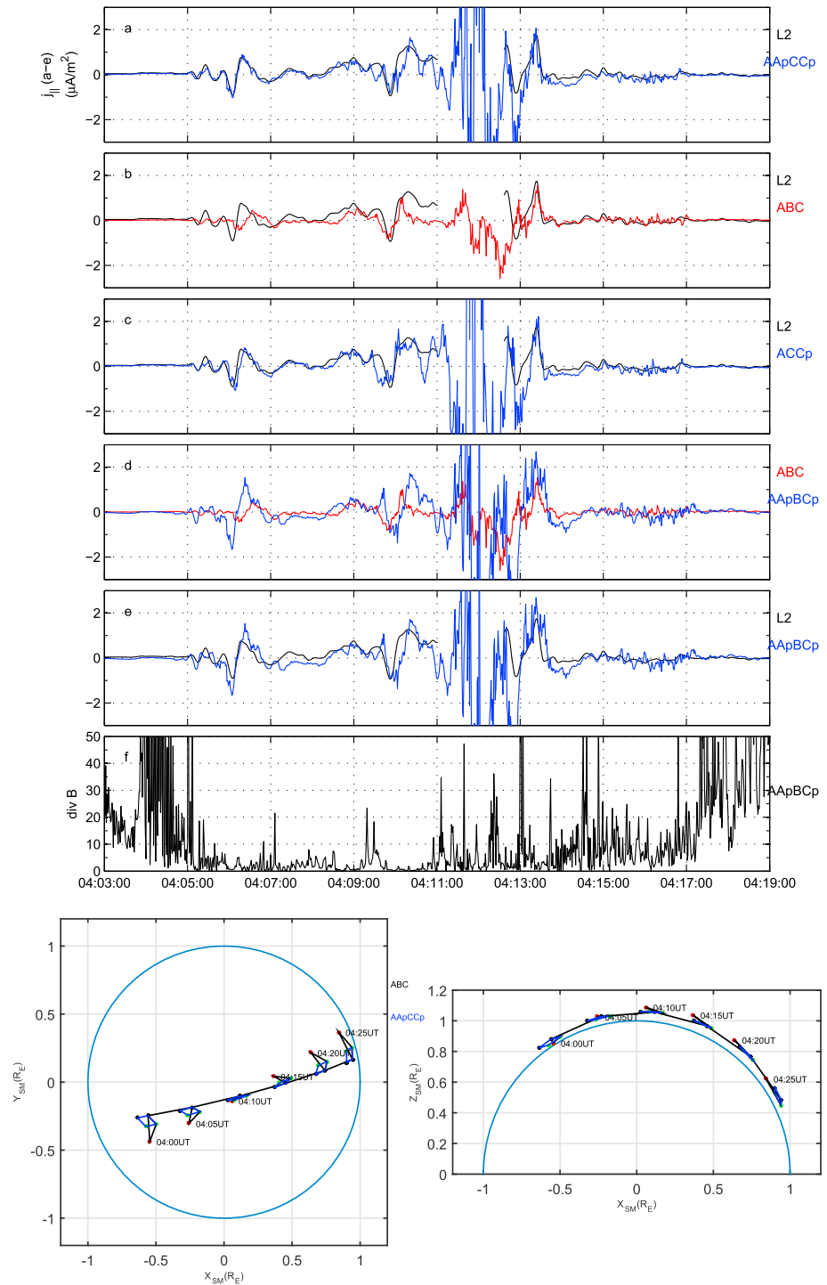
Figure 2. A set of curlmeter comparisons, for the data collected during 22 April 2014: (top, a) the unsmoothed estimate using positions AApCCp, compared to the smoothed level 2 (L2) data product; (b) the three-spacecraft spatial array, using ABC (i.e., no time shift, pure gradient calculation, which has a different J_N direction), compared to the L2 estimate; (c) 3-point formation, ACCp, compared to the L2 estimate; (d) comparison of the 4-point array (AApBCp) with the (e) ABC and L2 estimates, respectively; and (f) the ratios of \text{div}\mathbf{B}/\text{curl}\mathbf{B} (labelled \text{div}\mathbf{B} for short) for the 4-point estimate. (bottom) The orbit views ((right) X- Y_{SM} and (left) X- Z_{SM} ) show enlarged (5X) configurations as the Swarm spacecraft flew over the auroral zone and polar cap.
