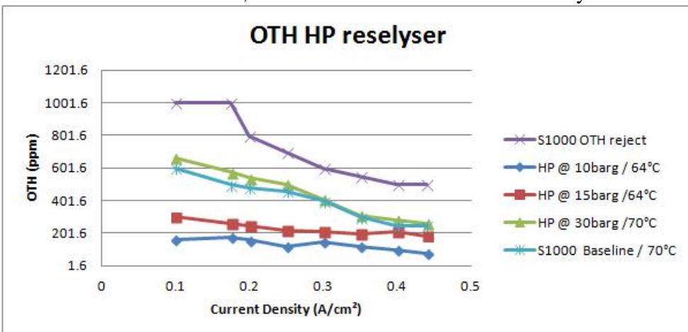
Figure.16: Oxygen content of the raw hydrogen stream of the HP stack at different pressures compared to the single membrane baseline (25 bar).
