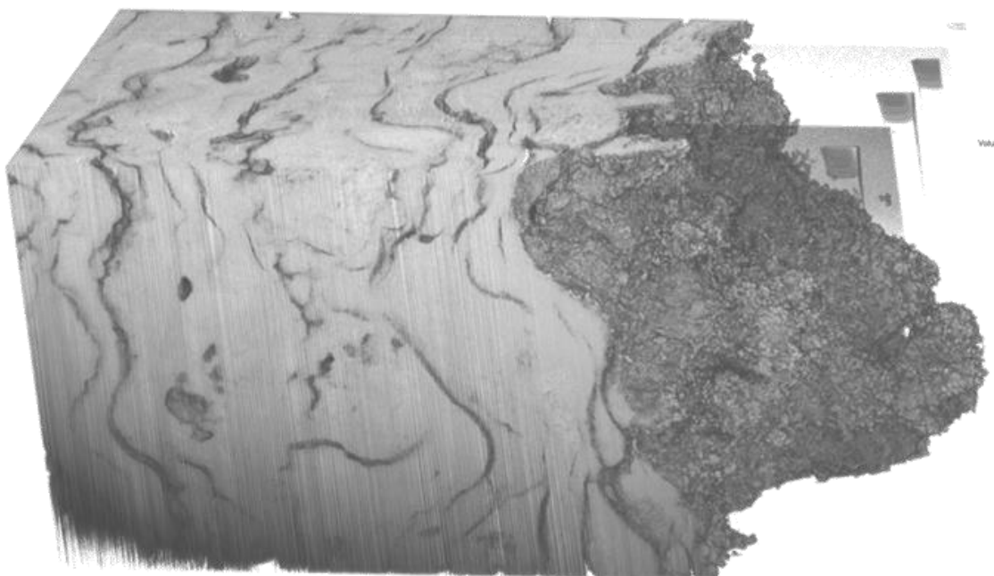
Figure 4: Three dimensional reconstruction of a tested cathode by focused ion beam tomography revealing surface topography (right side) and coarse scale internal porosity. Volume dimensions 75 x 30 x 45 \mu\text{m} (note: top right corner features are image processing artefacts).
