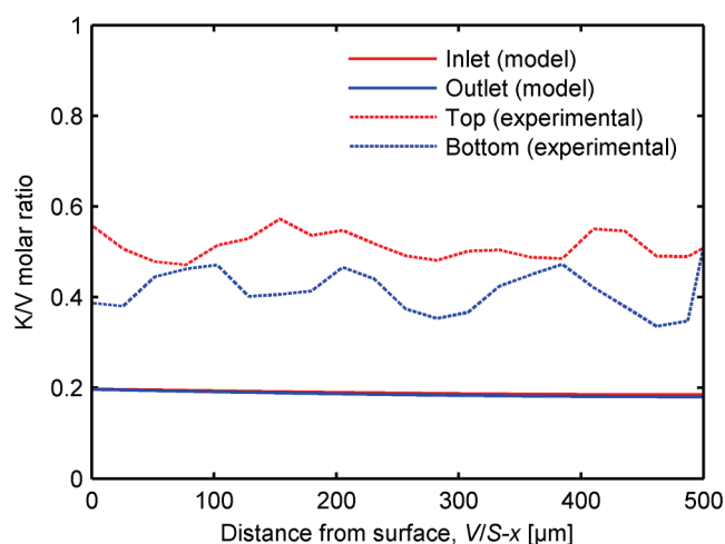
Figure 7.9: Simulated and experimentally measured K/V molar ratios across the half thickness of the catalyst wall of a 3\% \text{V}_2\text{O}_5\text{-}7\% \text{WO}_3/\text{TiO}_2 monolith after 960 hours of KCl exposure (simulation #2).
