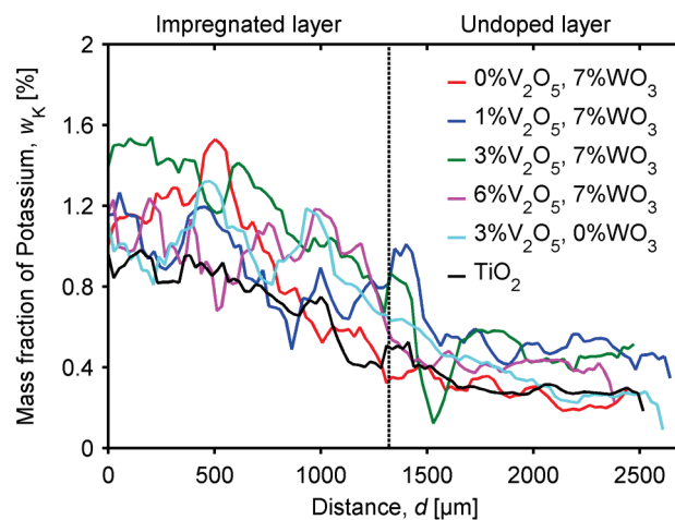
Figure 14. Potassium profiles in KCl impregnated (1.6 wt.% K, nominal) two-layer pellets of V_2O_5 - (WO_3) / TiO_2 catalysts, exposed to a flow (1000 NmL/min) of 6 vol.% O_2 and 3 vol.% H_2O in N_2 at 350 °C for 7 days.
