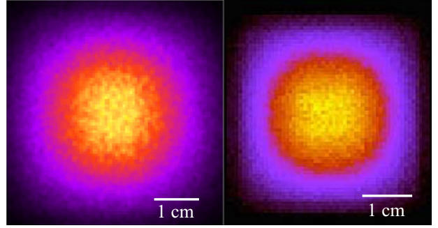
Figure 3. Beam profile at the sample position of the BASIS virtual instrument in McStas (left) and VITNESS (right) for a wavelength band of \Delta\lambda = 0.5 \text{ \AA} centred at \lambda = 6.4 \text{ \AA} . The area covered by the beam is approximately 9.6 \text{ cm}^2 . The colour scale was selected to allow easy comparison with results in the BASIS publication [14].
