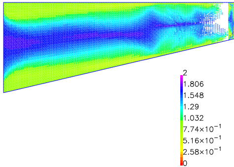
Figure 1: Visualization of distributions for constitutive matrices added direction of largest longitudinal stiffness in Figure 1a. The white spots near the tip of fixed material are places of minimum material density, being the same in all Figures 1a-d. The further white areas in Figure 1d contains materials classified as orthotropic.
