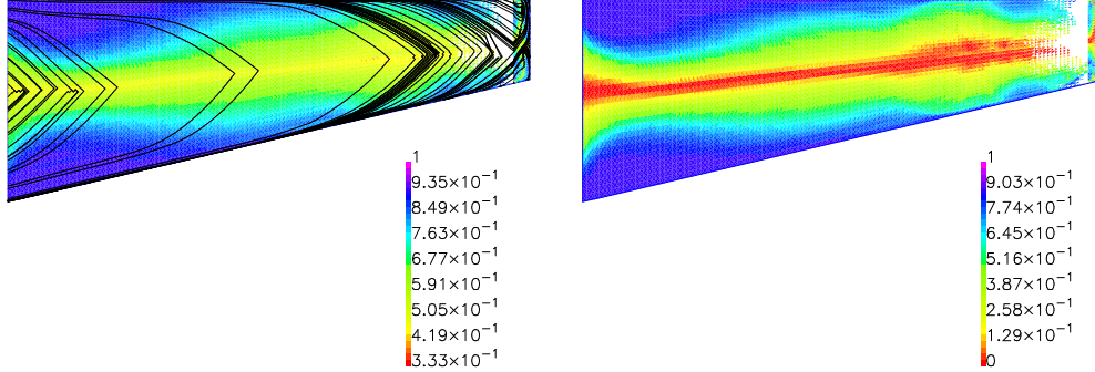
a) Largest longitudinal stiffness by (\alpha_{1111})_\theta b) Level of anisotropy by 2(\alpha_2)_\theta
