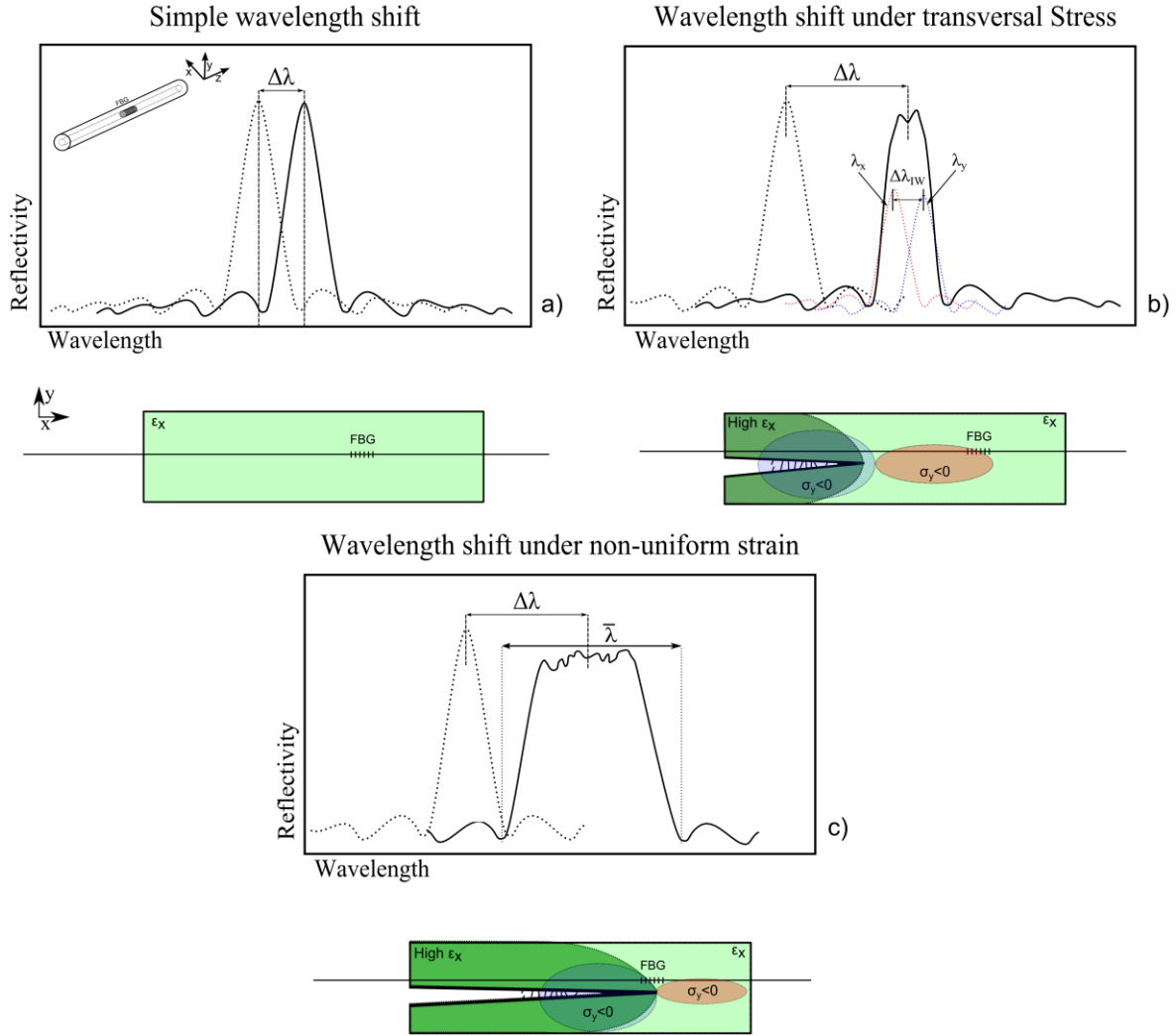
Figure 2: Different stages of the FBG response under a crack event.
