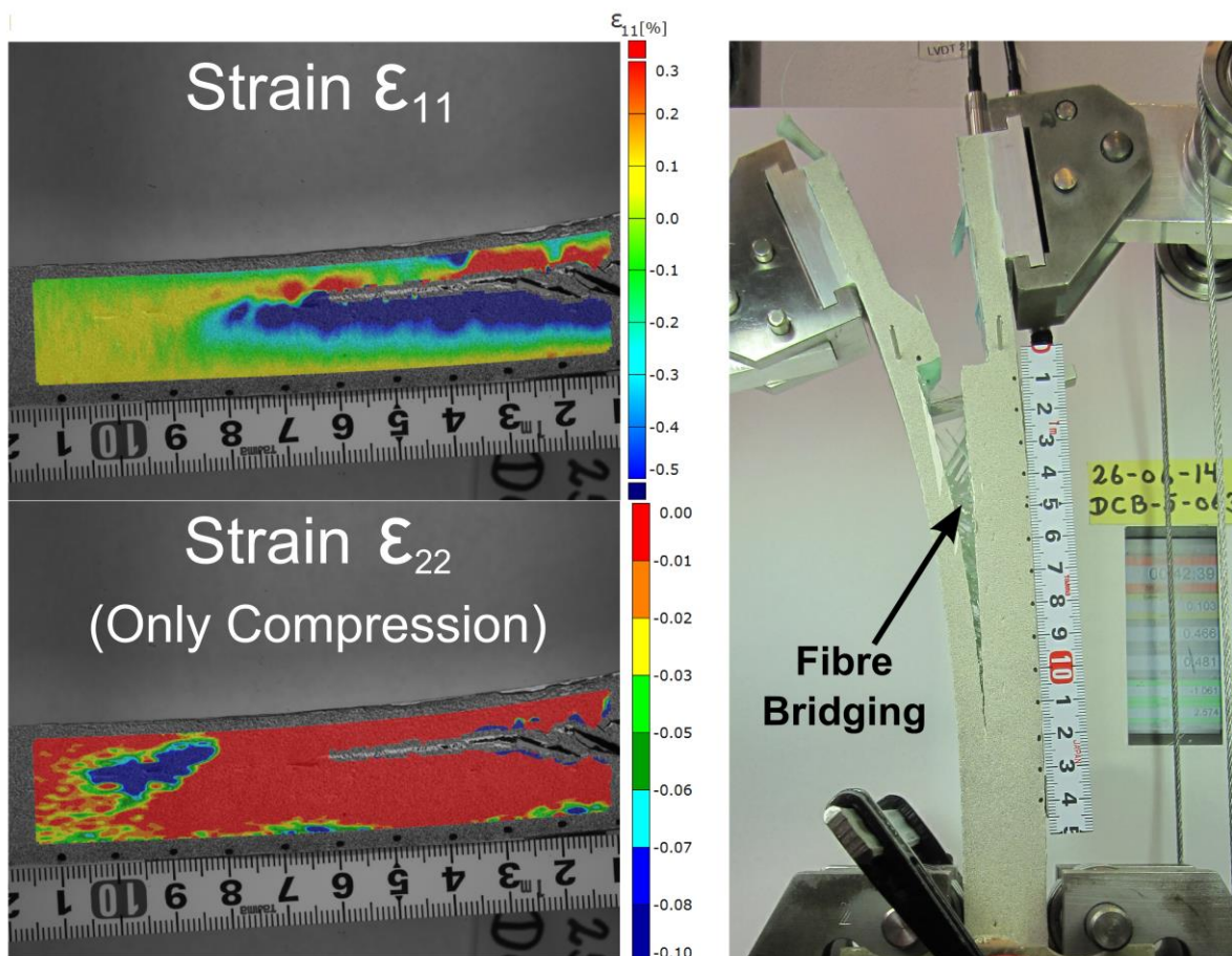
Figure 1: DIC measurement: strain distribution around a crack tip during delamination.
