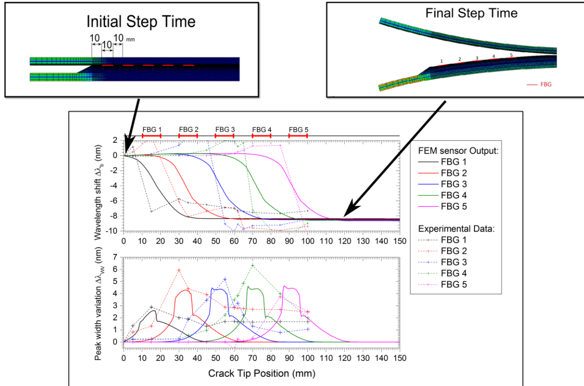
Figure 3: Model experimental validation: FBG Output prediction.
