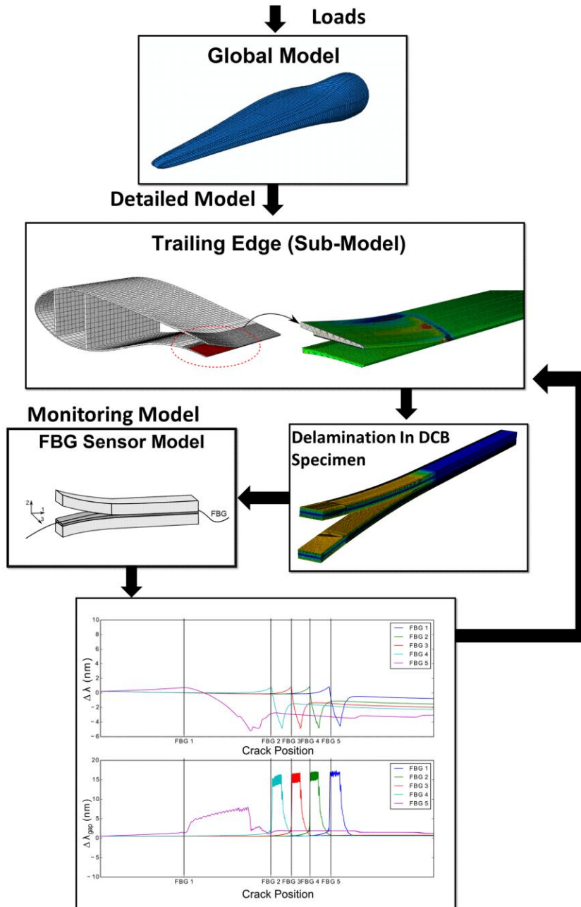
Figure 3: Model scheme of crack detection by embedded FBG sensors.
