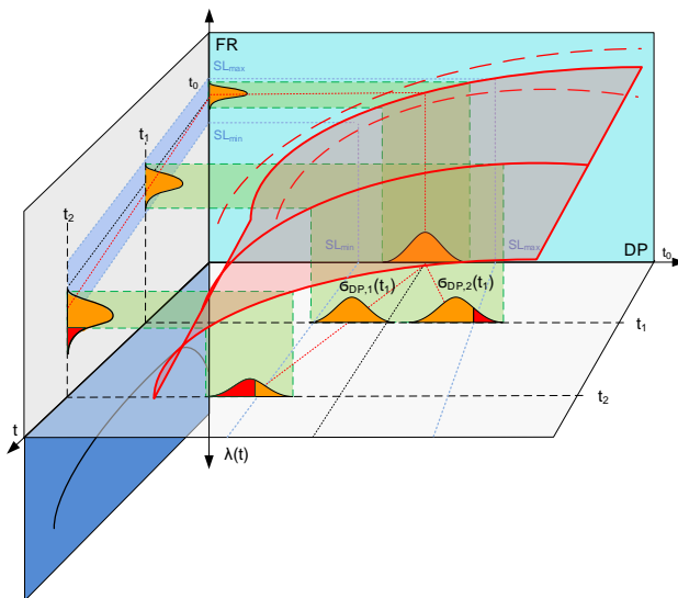
Figure 5: Integrated consideration of Reliability- and Robust Design theory
