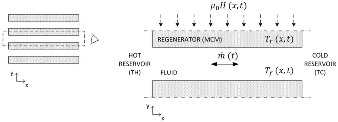
Fig. 1. Scheme of the 1D parallel-plate AMR model.
