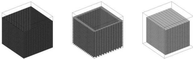
Fig.3. Three types of mesh elements in the imaging domain. From left: tetrahedra, prisms and hexahedra.
