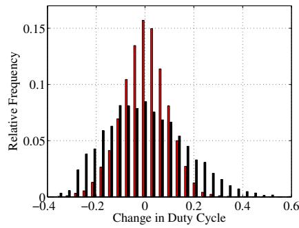
Figure 3.10: Relative frequency of duty cycle of ARMA (salmon colored) and measured data (black) over the 9 day validation data set. The duty cycle is plotted relative to the steady-state duty cycle. The ARMA model has more narrow, and more symmetric duty cycle changes than the measured data.
