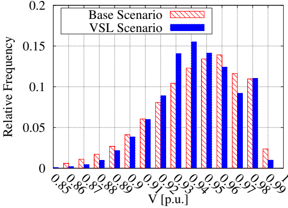
Figure 13. Distribution of voltage measurements in base case and VSL scenario.
