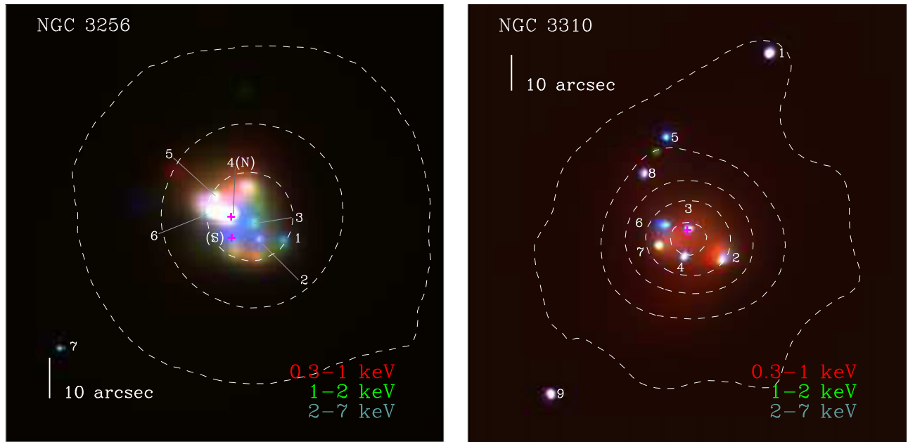
Figure 3. Three-color adaptively smoothed Chandra images of NGC 3256 and NGC 3310 with 4–25 keV NuSTAR intensity contours overlaid (dashed curves). The three bandpasses, 0.3–1 keV (red), 1–2 keV (green), and 2–7 keV (blue) were chosen to highlight the diffuse components from hot gas and unresolved point sources, as well as absorption in the bright point-source populations. A 10 arcsec bar has been added to each figure for reference. The annotated source numbers, ordered by increasing R.A., highlight bright point sources that are studied in Section 4.3 and presented in Table 2. The locations of galactic nuclei are indicated with magenta crosses. For NGC 3256, the northern (N) and southern (S) nuclei are labeled. With Chandra , we detect the northern nucleus of NGC 3256 (source 4, left) and the nuclear region of NGC 3310 (source 3, right). The NuSTAR FWHM is \approx 18 arcsec, which is sufficient for resolving some structure in the nearer NGC 3310; however, the NuSTAR emission for NGC 3256 is consistent with a single source PSF.
