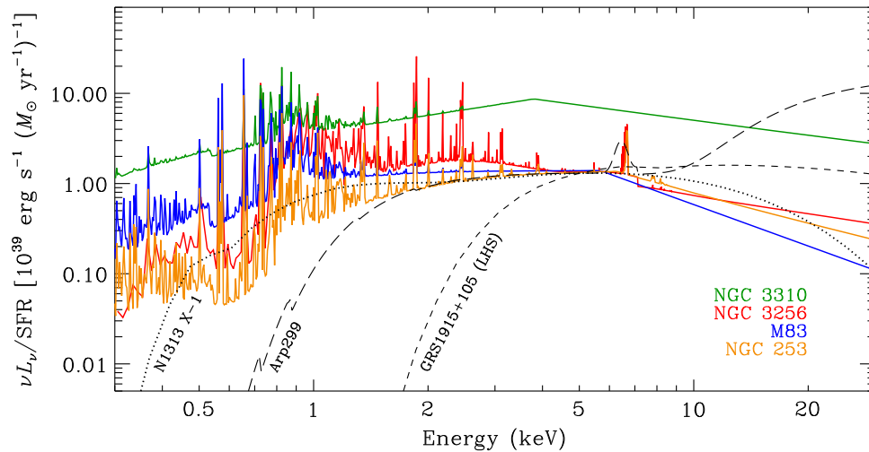
Figure 6. SFR-normalized 0.3–30 keV SEDs for NGC 3256 (red), NGC 3310 (green), NGC 253 (orange), and M83 (blue). For illustrative purposes, we have displayed only the best-fit SEDs to the nearly simultaneous Chandra/XMM-Newton plus NuSTAR data. NGC 253 and M83 fits are taken from the best-fit models presented in Wik et al. (2014a) and Yukita et al. (2015, in preparation). For comparison, we have shown NuSTAR constrained SEDs for the ULX NGC 1313 X-1 (dotted curve; Bachetti et al. 2013), the luminous black hole X-ray binary GRS 1915+105 in the low/hard state (short-dashed curve; Miller et al. 2013), and the Compton-thick AGN in Arp 299 (long-dashed curve; Ptak et al. 2014); these SEDs have been normalized to \nu L_\nu/\text{SFR} = 1.3 \times 10^{39} \text{ erg s}^{-1} (M_\odot \text{ yr}^{-1})^{-1} at 5 keV for ease of comparison. In this representation, a power-law SED with photon-index \Gamma = 2 is a flat line. It is clear that all four galaxies here show steepening in their SEDs above \approx 3\text{--}6 keV, where their spectral slopes reach \Gamma \approx 2.5\text{--}3.0 due primarily to the ULX population. These constraints indicate that the ULX population on average has a similar spectral shape to that of super-Eddington accreting sources like NGC 1313 X-1.
