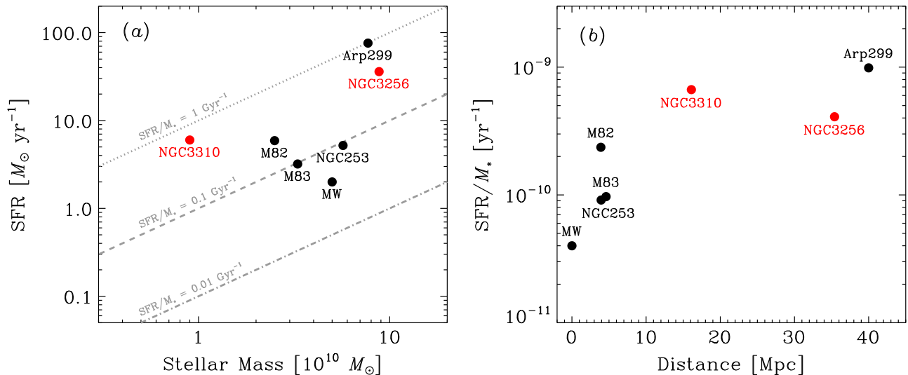
Figure 1. Physical properties of NuSTAR starburst galaxies sample. (a) SFR vs. M_* for the full sample with regions of constant specific SFR ( \text{sSFR} \equiv \text{SFR}/M_* ) highlighted. (b) \text{sSFR} vs. distance for the full sample. For comparison, the location of the Milky Way (MW) has been indicated. Our sample consists of galaxies with \text{sSFR} s that range from being comparable to those of the MW to a factor of \approx 20 times higher. We therefore expect that the X-ray emitting point-source populations in our sample will be skewed toward including richer populations of HMXBs compared to the MW (e.g., Lehmer et al. 2010; Mineo et al. 2012a). NGC 3256 and NGC 3310 are among the highest \text{sSFR} galaxies in our sample.
