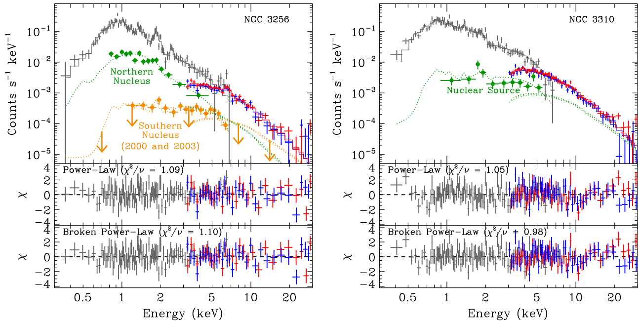
Figure 4. Joint nearly simultaneous Chandra (gray) and NuSTAR (red for FPMA and blue for FPMB) spectra for the full galactic extents of NGC 3256 (left) and NGC 3310 (right). The diffuse emission that is spatially isolated with Chandra was used to constrain two-temperature thermal ( apecc ) models for both galaxies. For NGC 3256, an additional obscured thermal component ( \approx 1 keV) was added to account for hot gas emission associated with the nuclear starburst. Absorbed single and broken power-law models that account for the Chandra -detected binaries were both tested for each galaxy, and the resulting residuals are displayed, and goodness-of-fit values are annotated, in the bottom two panels of each plot. We find that a single power-law is sufficient to fit the non-thermal emission from NGC 3256, while a broken power-law is preferred in the case of NGC 3310. We also display the contributions from nuclear components of these galaxies, with extrapolations to the NuSTAR band. For NGC 3256, this includes contributions from two nuclear regions associated with two galaxies in the merger: the northern nucleus contribution (green curve) and the estimated upper limit to the southern nucleus contribution (orange curve). The southern nucleus was not formally detected in our 2014 observation, and the upper limit spectrum here indicates the average Chandra spectrum from deeper observations in 2000 and 2003 scaled to the upper limit flux of our 2014 observation. We note that the southern nuclear region of NGC 3256 and the nuclear region of NGC 3310 both have flat X-ray spectra and are candidate low luminosity AGN (see Section 4.3 for details).
