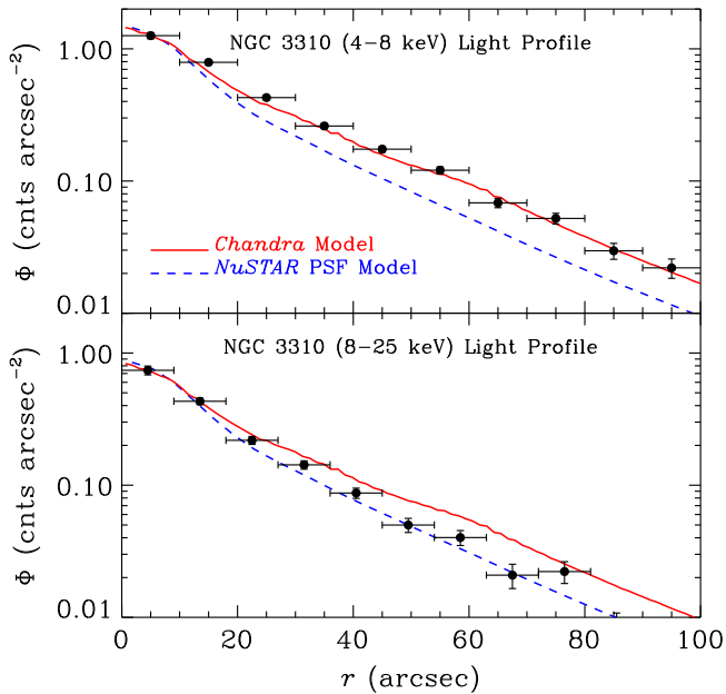
Figure 5. NuSTAR light profiles for NGC 3310 in the 4–8 keV (top) and 8–25 keV (bottom) bands. A blurred PSF model (blue dashed curves) and a model based on the relative 4–8 keV Chandra point-source brightnesses (“ Chandra Model ”; red solid curves) have been compared with the NuSTAR light profiles (black points). We find that the “ Chandra Model ” characterizes well the NuSTAR galaxy light profile in the Chandra and NuSTAR overlapping 4–8 keV bandpass. However, due to the presence of harder sources in the central region of the galaxy, as compared with sources in the outskirts, the 8–25 keV light profile becomes more point-like. Such a result could be explained by the presence of an obscured AGN and/or harder ULXs in the central region of the galaxy.
