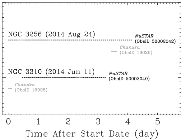
Figure 2. Relative NuSTAR (black lines) and Chandra (gray lines) observational coverage for NGC 3256 (top) and NGC 3310 (bottom). For clarity, we have annotated the starting date of the observational epoch. The apparently broken up NuSTAR observational intervals are due primarily to Earth occultations and passages through the SAA, which result in observing efficiencies of \approx 51\% – 58\% on average.
