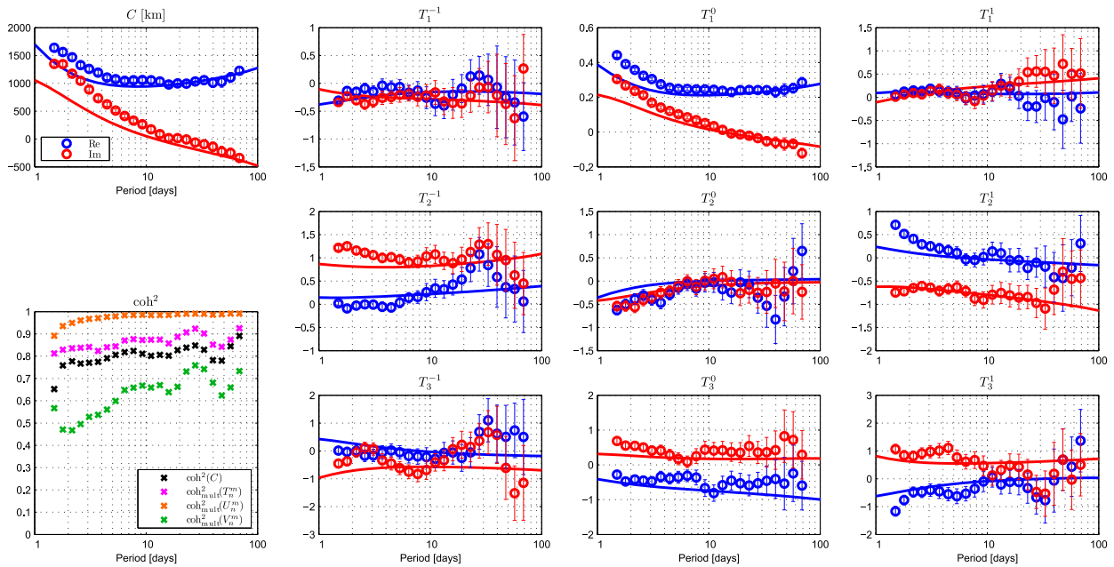
Figure 7. Transfer functions estimated for the observatory Hermanus (HER, South Africa) at geomagnetic latitude of 34^\circ\text{S} . The top panel in the first column shows C -responses. The bottom panel in the first column shows squared coherencies for C and multiple squared coherencies for the alternative transfer functions T_n^m , U_n^m and V_n^m . The further panels show the transfer functions T_n^m ( n \leq 3 , m \leq 1 ). For all responses, the real part is presented in blue, the imaginary part in red. The 90 per cent confidence interval is indicated for each estimate. Modelled transfer functions, corresponding to the conductivity model shown in Fig. 2, are marked by solid lines.
