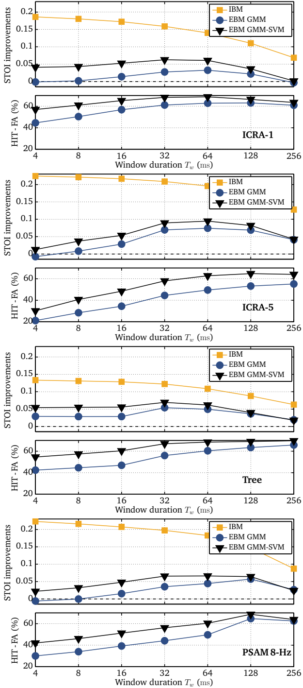
Figure 2: STOI improvements for the IBM and two EBM systems along with their corresponding HIT-FA rates averaged across all sentences and SNRs. The results are shown separately for each of the four noise types.
