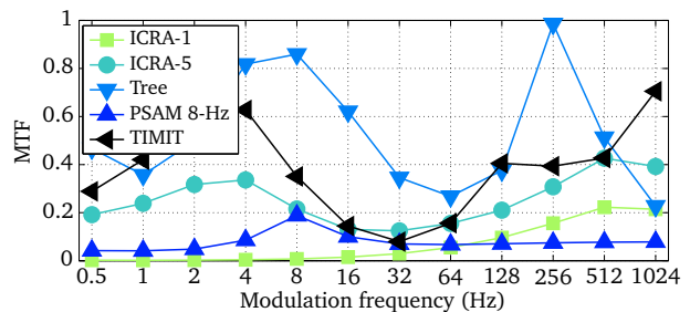
Figure 1: MTF of the four different background noises and the speech material from the TIMIT database.
