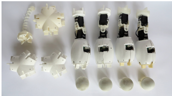
(a) Modules
