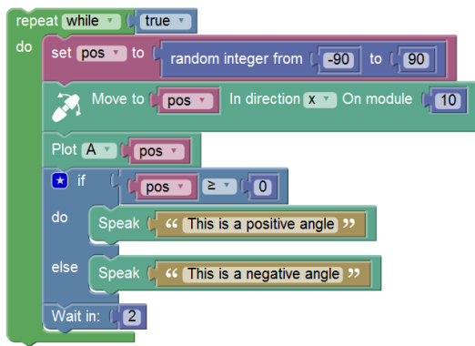
(a) Blockly
