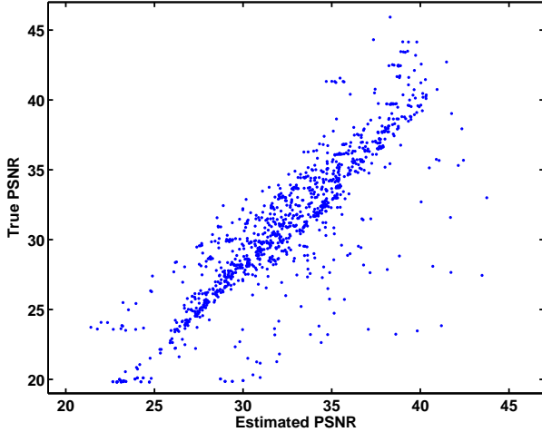
Fig. 8. Scatter plot of the PSNR estimation for analyzed frames in the Lisbon database. SROCC: 0.87.
