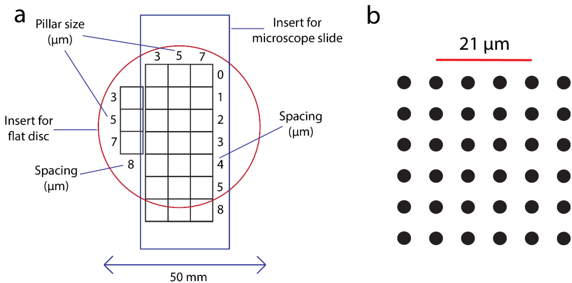
Figure 4.3. Mask design for pillar based structures; a) Mask layout pillars b) Arrangement of pillars with 3.00 \mu\text{m} in diameter and a spacing of 4.00 \mu\text{m} .
