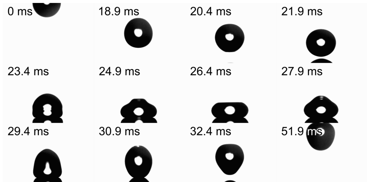
Figure 7.5. Image sequence showing a 6.5 µL drop impacting the structured polymer surface. At time zero, the drop is hanging from a needle, after 51.9 ms the drop have reached its maximum altitude after impact.
