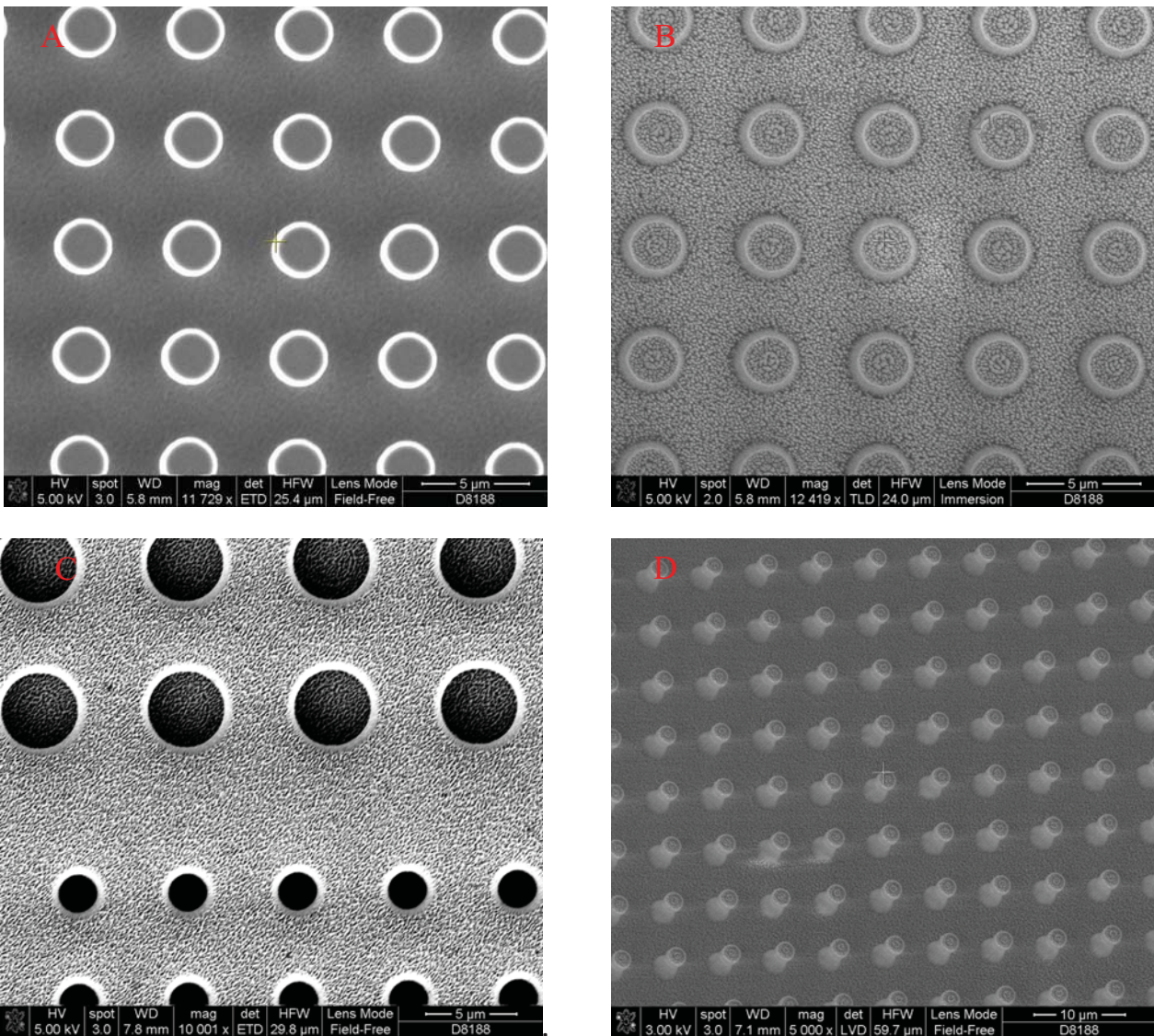
Figure 3: SEM images of different steps in the fabrication process. A) Micro pillars etched in silicon. B) Etch of hierarchical black silicon. C) Electroplated nickel insert with inverse structures. D) Injection molded self-cleaning surface hierarchical structures.
