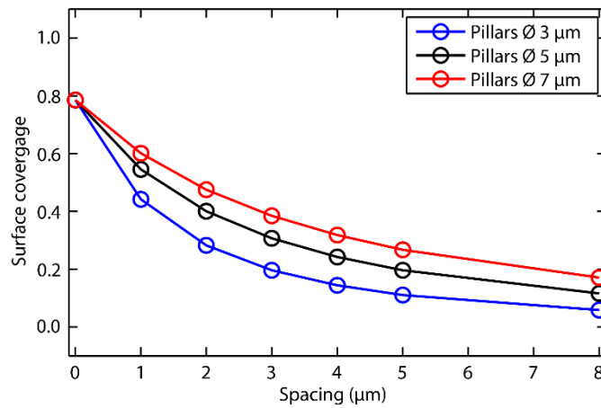
Figure 4.2. Surface coverage of pillars as function of spacing 3.00 \mu\text{m} , 5.00 \mu\text{m} , and 7.00 \mu\text{m} in diameter.
