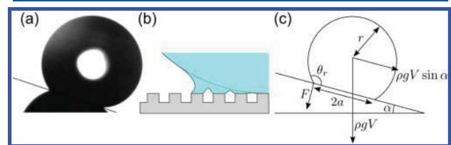
Figure 4. Graphical illustration of the model leading to eq 3. (a) Drop profile recorded with the camera on the contact angle goniometer at a tilt angle. (b) Sketch showing imagined formation of capillary bridges between the drop and the surface structure at the triple phase line. (c) Sketch of the drop geometry in the roll situation; the torque associated with the adhesion force F at the triple line is balanced by the torque associated with the gravity force \rho g V projected through the tilt angle \alpha .
