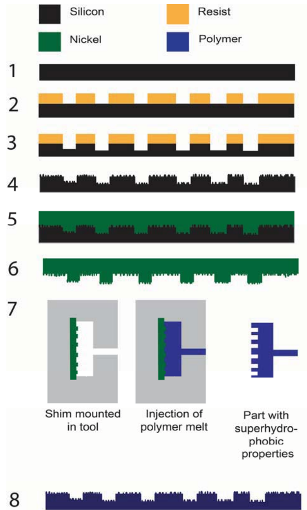
Figure 2: The entire fabrication method: 1 and 2) Lithography, 3) Dry etch, 4) resist strip and black silicon etch, 5) Electroplating of nickel shim, 6) removal of silicon wafer with KOH, 7) injection molding of polymer parts from nickel shim, 8) finished parts with super hydrophobic surfaces.
