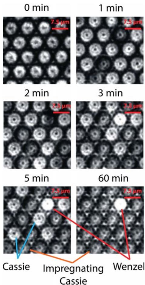
Figure 3. Optical transmission microscopy images of microcavities during water wetting experiments at \Delta p = 225 mbar. The colored lines indicate examples of different wetting states on the micrographs. To distinguish one state from the other visually on the images, the contrast on the images was increased (Supporting Information). 40
