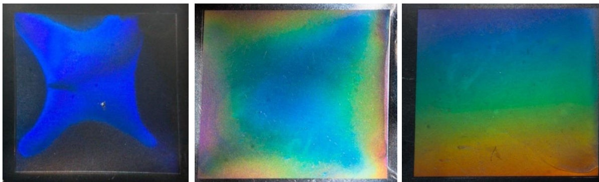
Figure 5.30. Filling of nanostructures Left: uneven filling (1400 bar/25 °C), Center: moderate filing, Right: even of filling (holding pressure and cycle time of 60 s).
