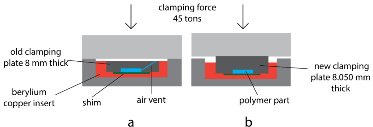
Figure 5.16. Thickness of the clamping plate was increased to prevent polymer leaking.
