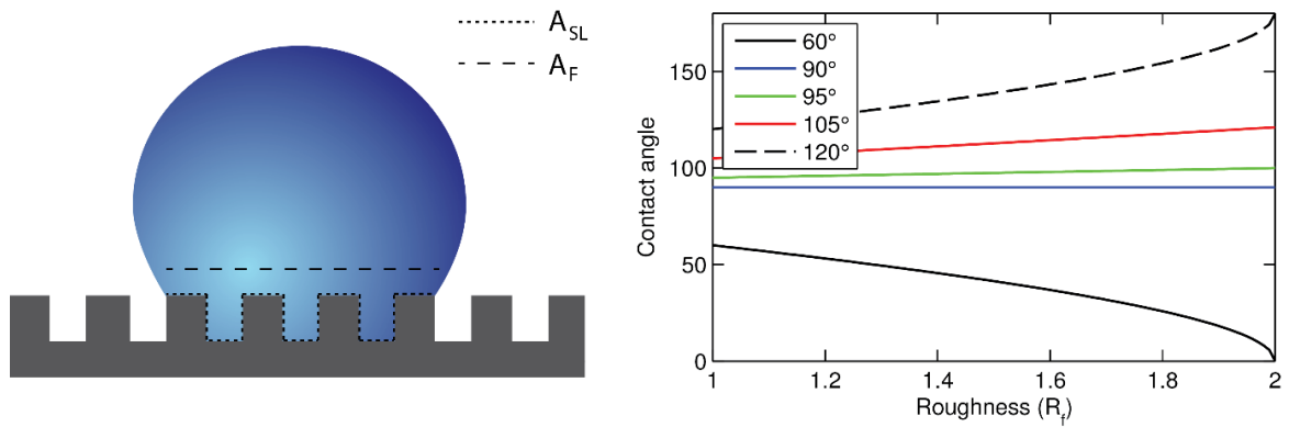
Figure 2.5. Wenzel State where the drop completely wets the surface roughness (which is schematically drawn as periodic structures). This is also known as the pinned state. A_{SL} are the total surface area and A_F the area projected by the drop. The plot shows the Wenzel equation with contact angle as function of roughness for different intrinsic contact angles.
