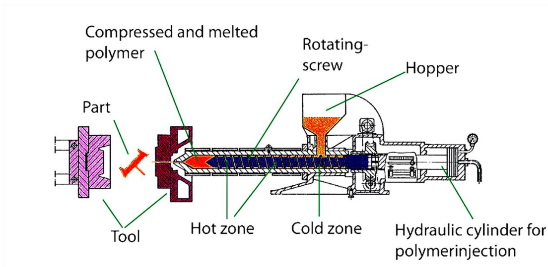
Figure 5.8. Schematically drawing of injection molding machine. Modified from 81 .
