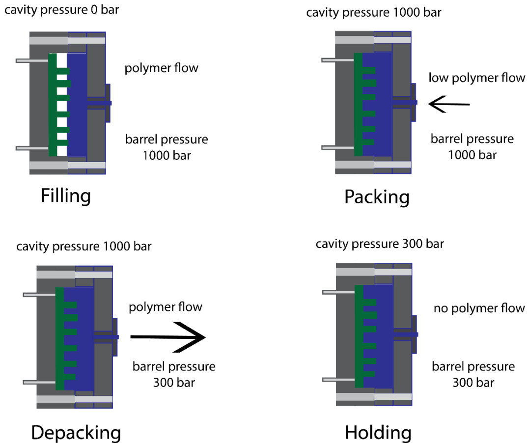
Figure 5.14. Principle of the depacking phase. A high packing pressure fills nano- and micro-structures. Depacking ensures that the part can be demolded.
