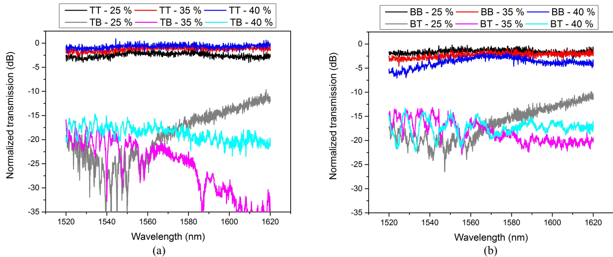
Figure 9: Spectra from the S2 structure optimized with a resolution of 16 nm for three different choices of structural threshold values. (a) Spectra of the TE 0 -TE 0 -TE 0 conversion and (b) of the TE 0 -TE 1 -TE 0 conversion. Data is normalized to the TE 0 mode of a single mode waveguide with the same length and bends at input and output.
