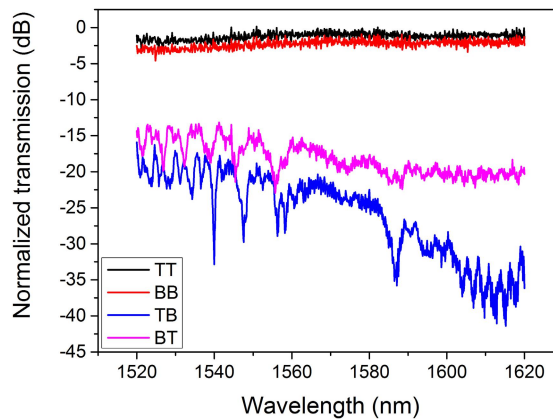
Figure 8: Normalized transmission spectra of the S2 structure optimized with a resolution of 16 nm and extracted with a threshold of 35 %. Spectra are normalized to the TE_0 mode of a single mode waveguide with the same length and bends at input and output.
