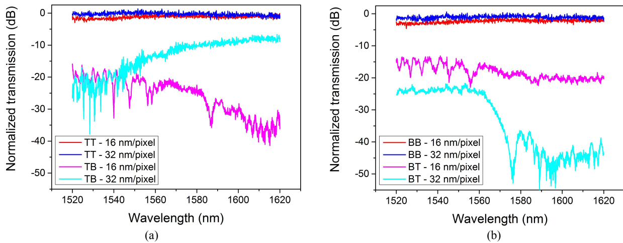
Figure 10: Measured spectra of the S2 structure with a threshold of 35 % and designs optimized with different resolutions. Measured spectra for light following (a) a TE 0 -TE 0 -TE 0 path and (b) a TE 0 -TE 1 -TE 0 path. Data is normalized to the TE 0 mode of a single mode waveguide with the same length and bends at input and output.
