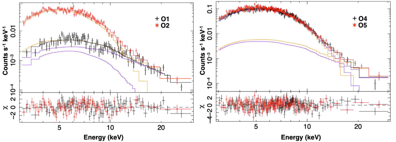
Figure 4. Spectra of the outburst phases with their best-fit model and the decomposition of the model into the blackbody component and the power-law component (high-energy tails). The left panel shows the spectrum of phases O1 (black plus signs, and model breakdown in purple), and O2 (red crosses, and model breakdown in orange). The right panel shows phases O4 (black plus signs, and model breakdown in purple) and O5 (red crosses, and model breakdown in orange). Each spectrum is the combination of data from modules A and B. The data points are shown with 1\sigma error bars, and the solid lines show the best-fit model. The lower panels show the deviation from the model in units of standard deviation.
