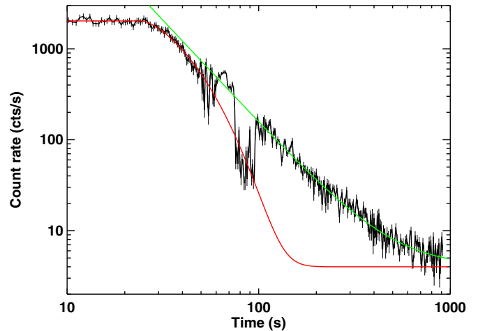
Figure 3. Burst decay light curve in the 3–30 keV band, with 0.5 s, 1 s, 2 s, 4 s, and 8 s bins, in the 0–60 s, 60–120 s, 120–240 s, 240–480 s, and 480–1000 s ranges, respectively. The red curve shows the modified FRED curve fit to the 0–50 s interval of the light curve (identical to the model presented in Figure 2), and the green curve shows a power-law fit to the 110–900 s interval. Both models include a constant equal to 4 counts s^{-1} to account for the persistent emission.
