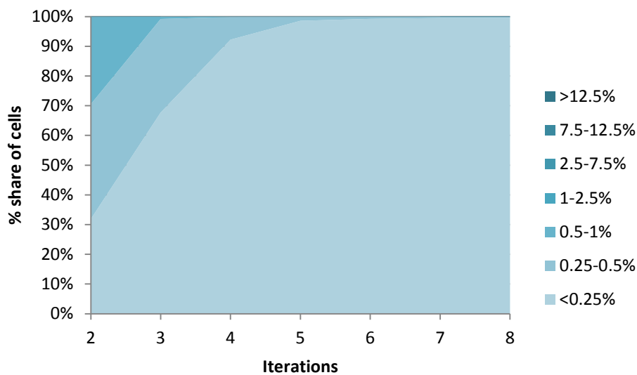
Figure 11. System convergence illustrated as a distribution of \mathbf{abs}\left(\frac{S(t_k)-t_k}{t_k}\right) for LoS and classified in seven deviation bands, with d = 1 and MSA by LoS.
