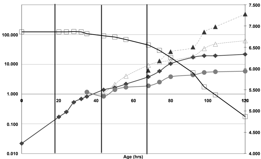
Figure 2b: Batch profile of a typical S. coelicolor oxp-ptpA cultivation in minimal medium, using microtiter plates. The graph shows time course measurement for OD_{450nm} (♦), DCW (■) g/L, ACT (▲) and RED (Δ) in mg/L, and pH (□). The three vertical lines from left to right indicate – start of exponential phase, onset of RED and ACT production, respectively. All the trends (OD, DCW, ACT and RED) except for pH trend are represented on primary axis.
