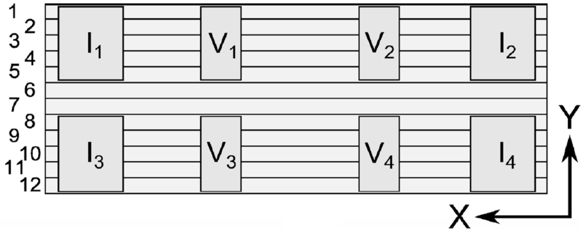
2 Figure 2. A schematic illustration showing positions of the current I_i and voltage V_i taps for the four-point 3 probe analysis of the 2LUPS CC, where i=1-4 . Labels 1 to 12 on the Y-axis indicate filament numbers, 4 where even and odd numbers correspond to lower and upper plateaus, respectively.
