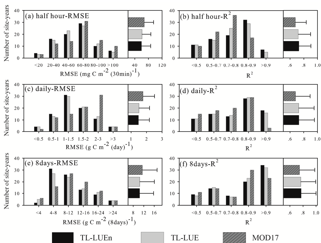
Figure 2. The number of site-years within different root mean square error (RMSE) and R^2 classes (left) and the averages of RMSE and R^2 (right) of GPP simulated using the TL-LUEn, TL-LUE, and MOD17 models in 85 calibration site-years at half-hourly (a,b), daily (c,d), and 8-day (e,f) temporal scales, respectively.
