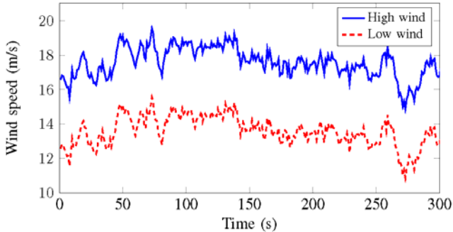
Fig. 3 Wind speed variation of WT 05
