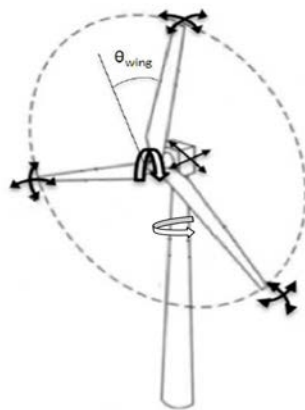
Figure 1. Degrees of freedom of the aero-elastic model.
