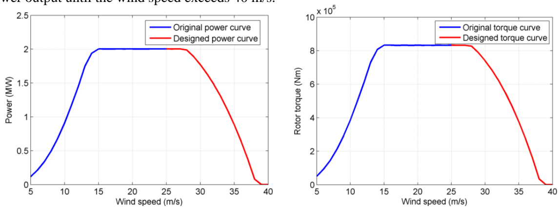
Figure 2. Redesigned power curve and torque curve from optimization.
