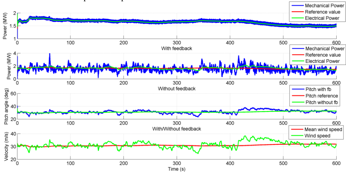
Figure 4. Power output and pitch angle of the wind turbine by feedforward control with/without feedback in high wind speed conditions.
