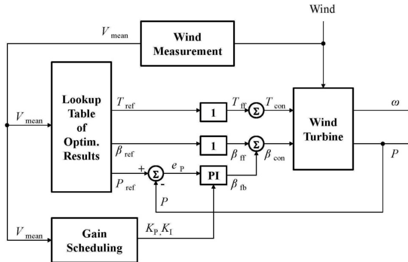
Figure 3. Control schema of the proposed control strategy.
