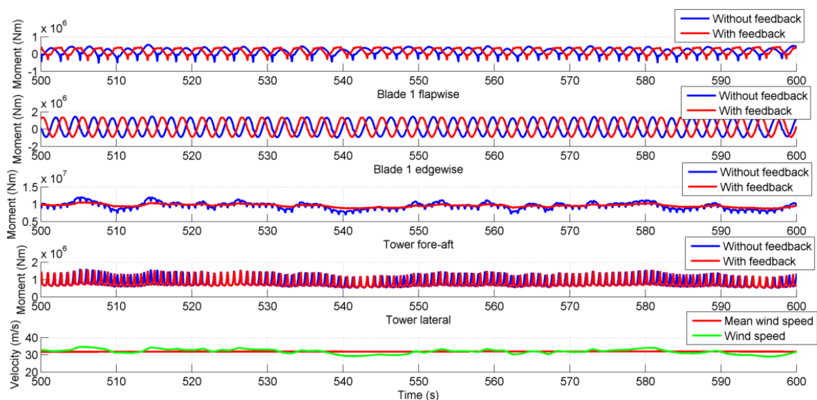
Figure 5. Blade bending moments and tower bending moments of the wind turbine by feedforward control with/without feedback in high wind speed conditions.
