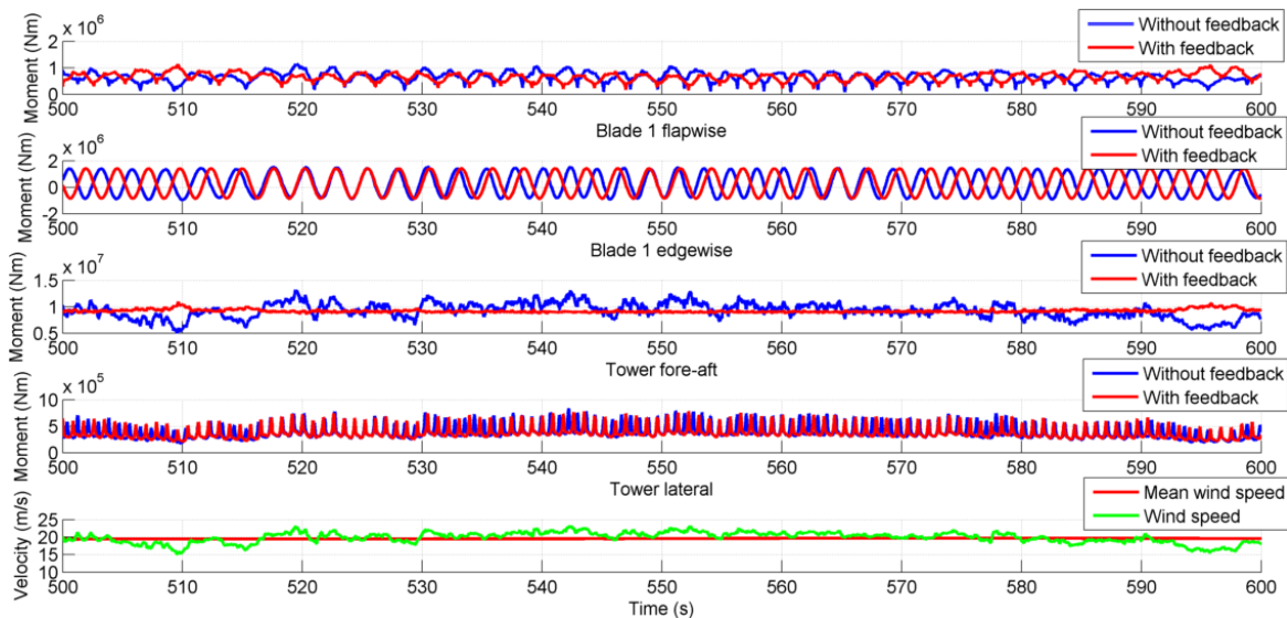
Figure 7. Blade bending moments and tower bending moments of the wind turbine by feedforward control with/without feedback in middle wind speed conditions.
