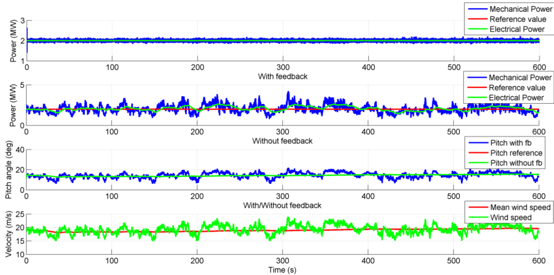
Figure 6. Power output and pitch angle of the wind turbine by feedforward control with/without feedback in middle wind speed conditions.
