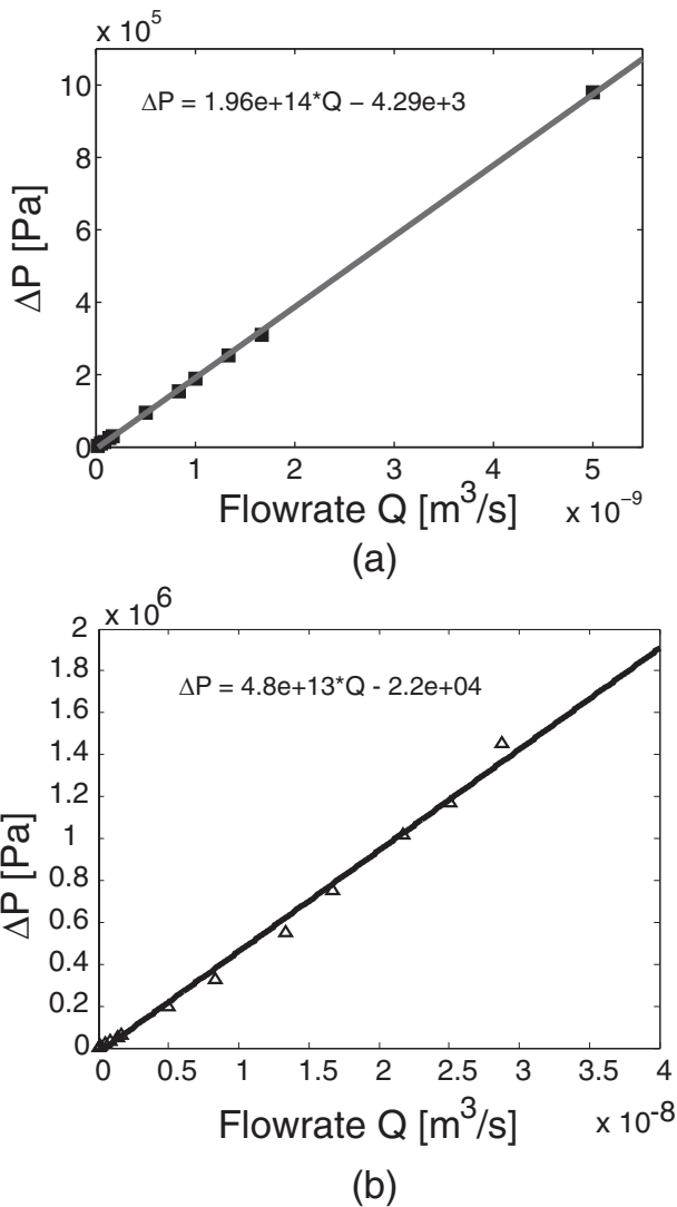
Figure 9. Pressure drop test after bonding (a) PI-PI bonded microfluidic channel with dimensions Length x Width x Height = 3118 x 77 x 22.9 μm (b) PI-glass bonded microfluidic channel with dimensions Length x Width x Height = 3118 x 77 x 11.6 μm.
