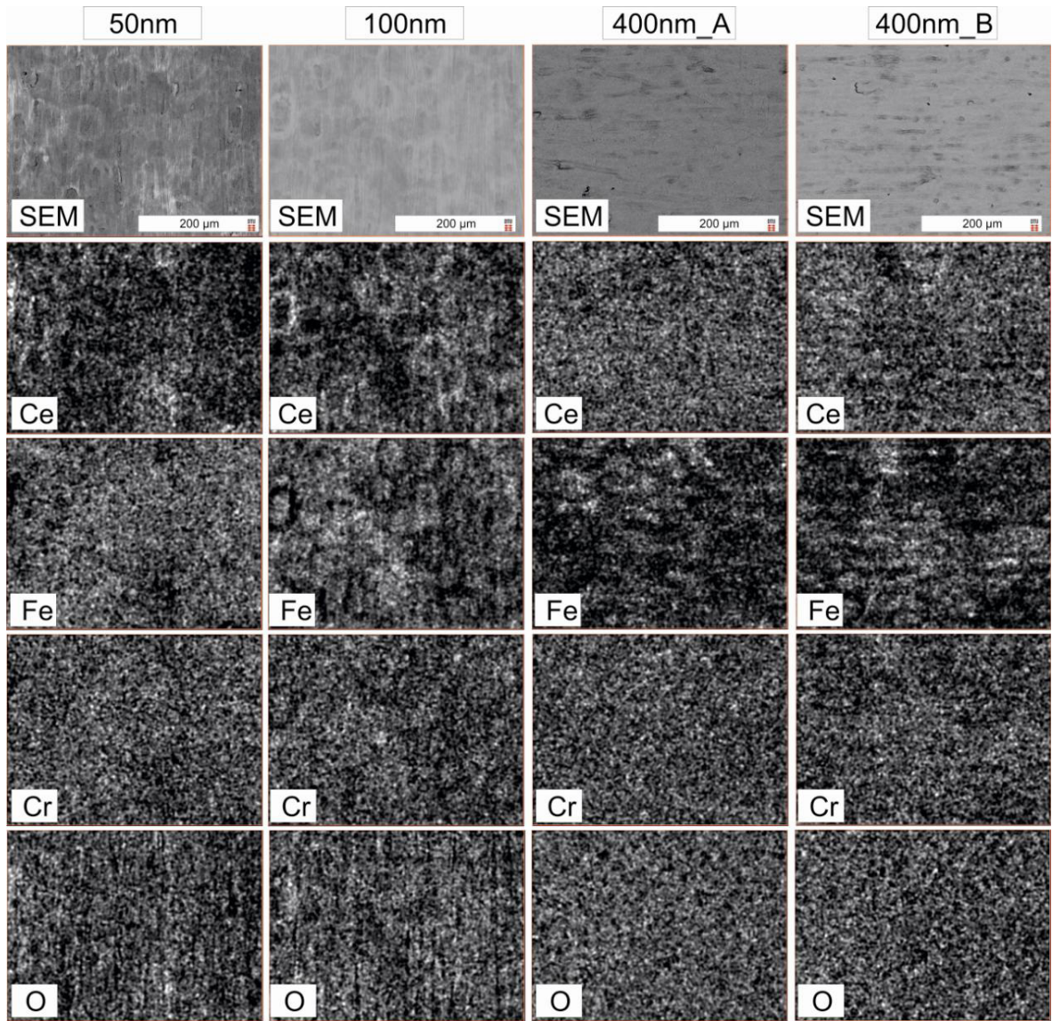
Figure 3. Energy dispersive x-ray spectroscopy elemental analysis of coated samples.
