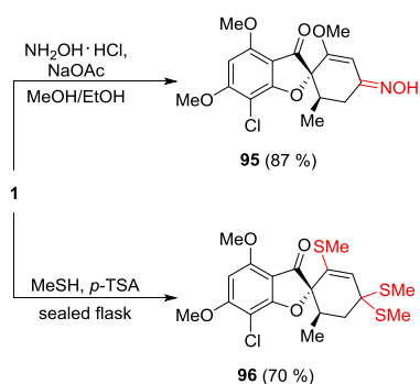
Scheme 21. 4'-Analogues prepared from griseofulvin 1 .
