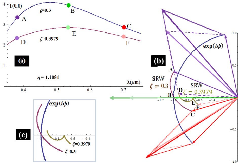
Fig. 2. Wavelength dependence using GPC parameters optimized for Gaussian-to-top-hat shaping at \lambda_0 = 532\text{nm} . (a) On-axis intensity vs wavelength shows that the efficiency optimized top-hat size ( \zeta = 0.3979 ) exhibits a flatter wavelength response than a smaller top-hat ( \zeta = 0.3 ). (b) Complex plane visualization illustrating how the phasors drift from as the wavelength changes. Phasor diagrams illustrate the on-axis output superposition [cf Eq. (6)] of the modulated Gaussian, \exp(i\phi) , with the corresponding SRW phasors for the two top-hats, marked \zeta = 0.3 and \zeta = 0.3979 , at selected wavelengths marked A–C (D–F) in (a). (c) Zoom-in of how the SRW phasors drift as the wavelength changes from A–C (D to F) for \zeta = 0.3 ( \zeta = 0.3979 ).
