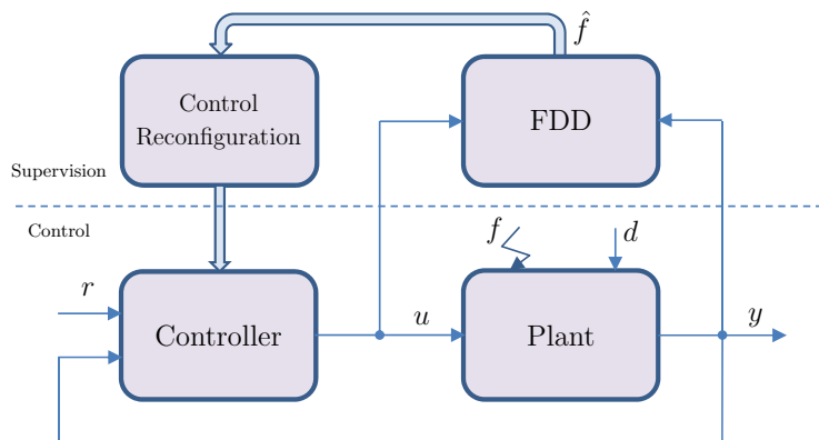
Figure 1: Structure of Active Fault Tolerant Control
