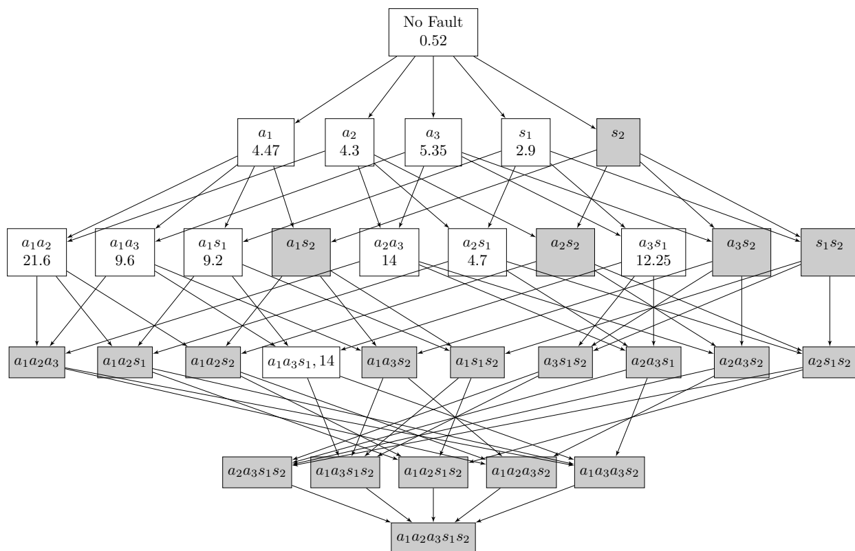
Figure 7: Lattice of system configurations for example 2, Each block represents a configuration where the corresponding component is failed.
