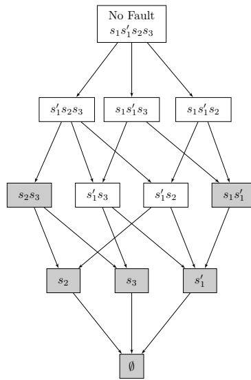
Figure 4: Lattice of system configurations for example 1 with redundant sensor for the first state
