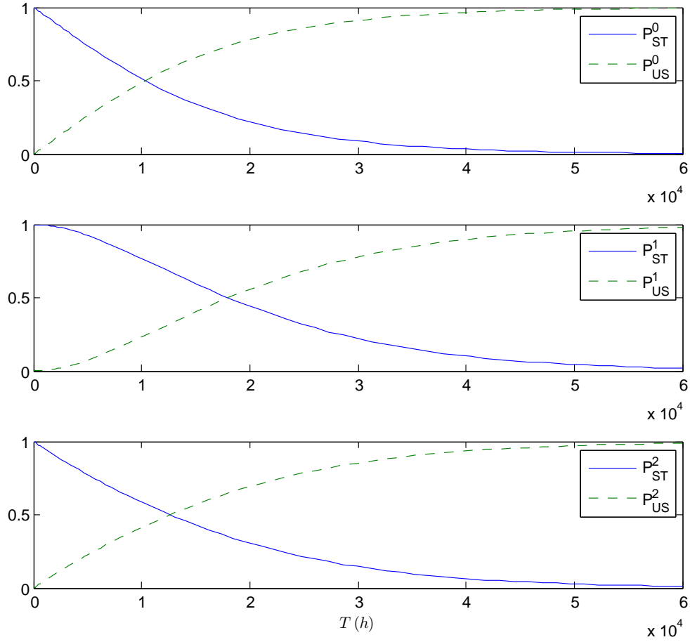
Figure 5: Probability of being in the stable ( P_{ST} ) and unstable mode P_{US} with different configurations: (Top row) one sensor for each state ( s_1s_2s_3 ), (Middle row) a redundant sensor for the first measurement ( s_1s'_1s_2s_3 ), (Bottom row) a redundant sensor for the third state ( s_1s_2s_3s'_3 )
