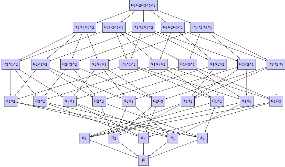
Figure 2: Lattice of possible configurations for a system with three actuators a_1, a_2, a_3 and two sensors s_1, s_2 . Moving from top of the diagram to its bottom represents the loss of components.
