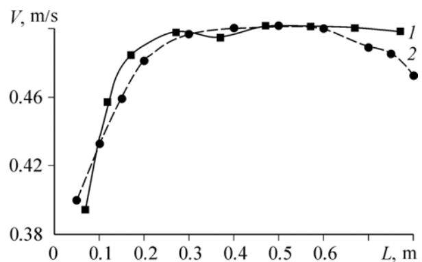
Figure 2. Examples of velocity profile from the wall (1) and the bottom (2) in cross sections of the flume.
