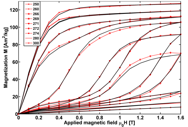
Fig. 1. Isothermal magnetization measurements on Gd_5Si_2Ge_2 (dashed symbols) and the corresponding Preisach model simulations (solid lines).
