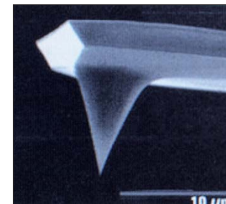
Vippearmen i et atomic force mikroskop.
