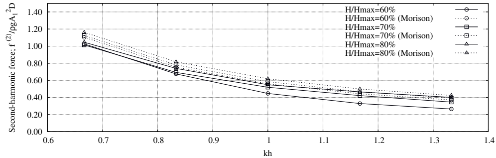
(b) Second-harmonic
