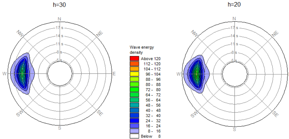
Figure 4: Test DirH4T14: Directional spectra obtained from MIKE 21 SW at two different depths.
