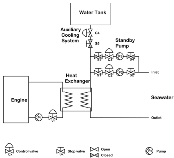
Figure 2. The ship engine cooling system
