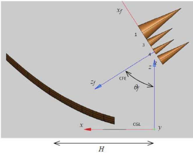
Figure 1. Optimized configuration of the mm-VAST antenna: CGL – global coordinate system, CFE – feed cluster coordinate system.
