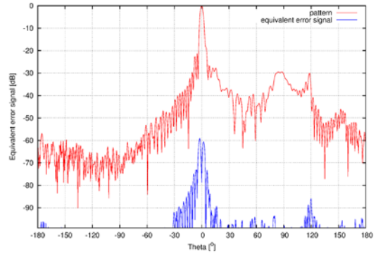
Figure 4. VAST-12 offset plane, 0.003^\circ displacement.
