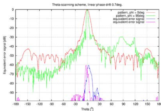
Figure 5. VAST-12, z -axis pointing, \theta -scan, 0.7^\circ phase shift.
