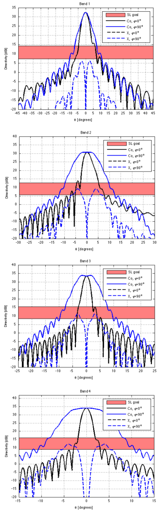
Figure 2. Simulated mm-VAST patterns for the LP.
