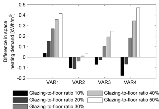
Figure 5: Differences in space heating demand for different variations in window distribution for an even window design.
