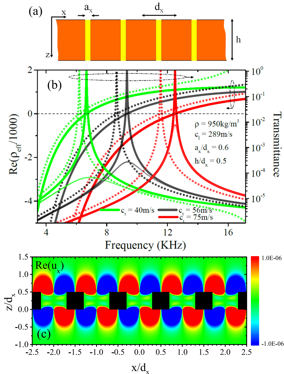
FIG. 1. Transmittance and effective mass density spectra of the (a) structured and elastically filled rigid screen surrounded by air. (b) In all three cases the geometries are the same, we only vary c_t as indicated. All calculations are undertaken for normally incident sound where the full (dotted) lines represent data obtained by modal expansions (COMSOL simulation). Transmittance containing dissipation have been simulated such that \text{Im}(c_t) = \text{Im}(c_l) (open circles). For the three plotted examples, from left to right in the spectrum we have chosen \text{Im}(c_t) = 10, 5 and 1 \text{ m/s} . (c) At f = 6 \text{ kHz} with d_x = 5 \text{ mm} and c_t = 40 \text{ m/s} we plot \text{Re}\{u_x\} . Color bar units are in m.
