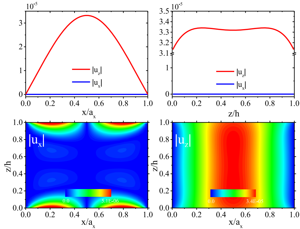
FIG. 2. From the previous example Fig. 1(c), we simulate the elastic displacements |u_x| and |u_z| within the filled aperture. In particular we plot these displacements across the aperture ( z/h = 0.5 ) and along ( x/a_x = 0.5 ). Notice the different magnitudes of the color bars. All units are in m.
