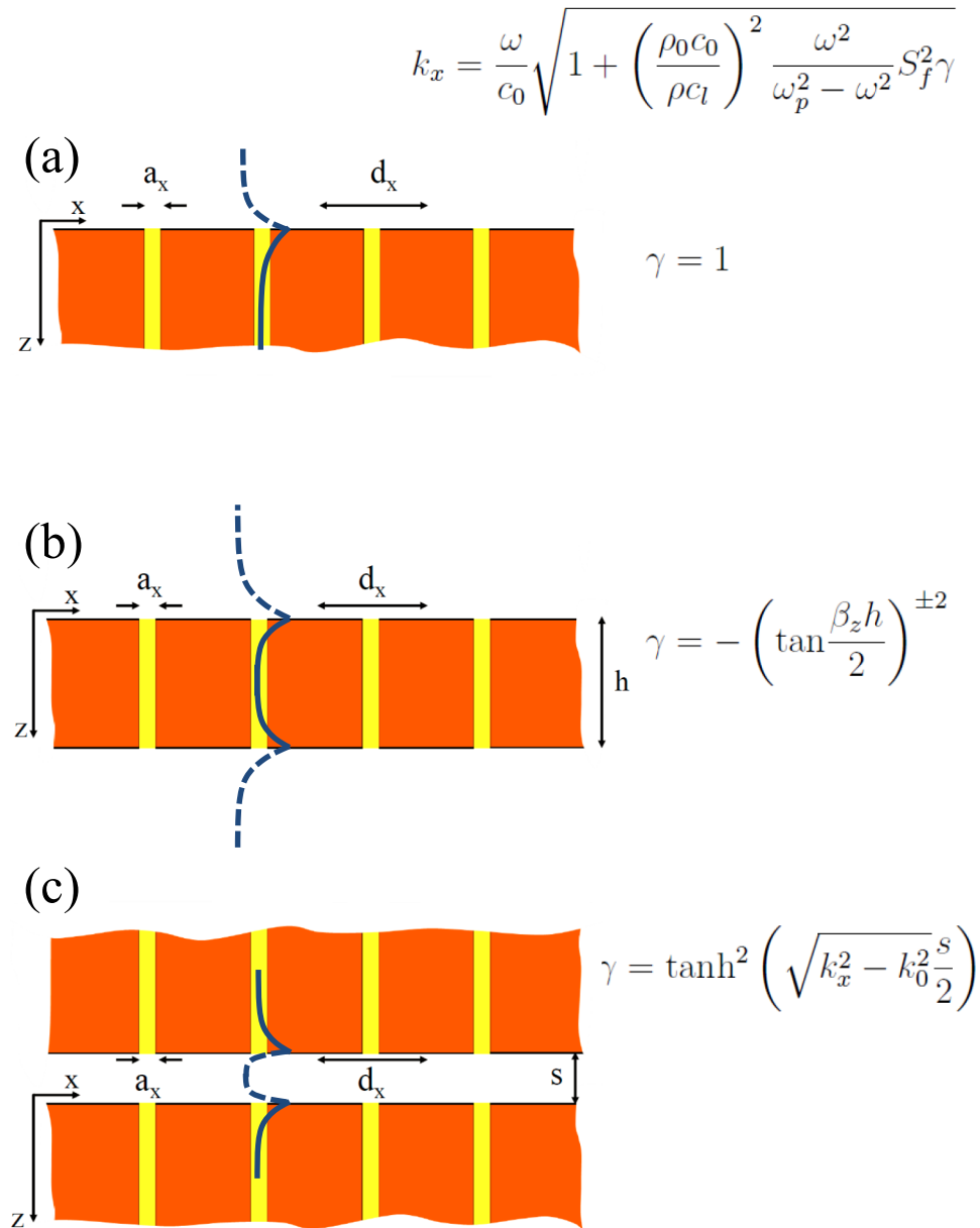
FIG. 3. Three different structured surface waveguides. We present the generalized dispersion relation for bound non-leaky modes. With corresponding coefficients \gamma representing the out-of-plane coupling, we illustrate surface waveguides in the form of a structured (a) half-space, (b) plate and (c) gap.
