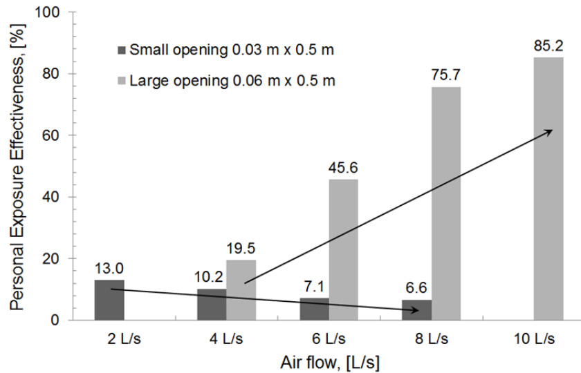
Figure 2. PEE as a function of flow rate. Both inner (PV air) and outer (room air) jets provide same amount of air
