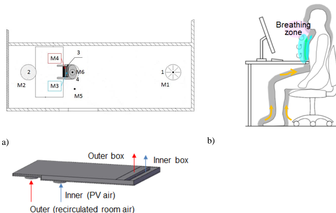
Figure 1. Set-up of the experiment with the confluent PV jet box a) chamber set-up and b) application of confluent jets as a table incorporated PV unit, c) confluent PV jet design, 1) TV supply, 2) TV exhaust, 3) confluent PV jet design, 4) breathing thermal manikin. With M are shown the tracer gas measurement locations: M1 – supply, M2 – exhaust, M3 – inner jet, M4 – outer jet, M5 – room and M6 – manikin mouth.
