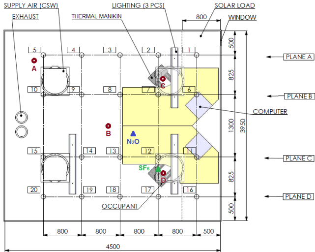
Figure 2: Experimental set up case “DC/CSW office 50 \text{ W}\cdot\text{m}^{-2\text{a}} and case “DC/CSW/ office 78 \text{ W}\cdot\text{m}^{-2\text{b}} ”. Mean air speed and mean air temperature measured in locations numbered from 1–20 (locations 6, 7, 11 and 12 excluded). Concentration of tracers gases measured in locations A–D (heights: A: 0.1, 0.6, 1.1, 1.7, 2.4 m, B: 0.1, 0.6, 1.1, 1.7, 2.4 m, C–D: 1.1 m).
