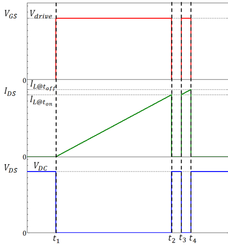
(b) Double pulse tester switching pattern
