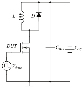
(a) Double pulse tester schematic
