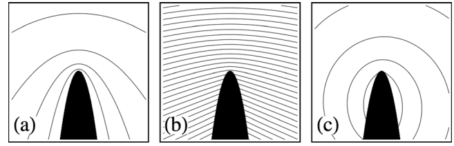
FIG. 5. (a) Tip (dark) and equipotential surfaces surrounding it, with a spacing of 1 V, based on the model described in the text, for input values of a = 0.97 mm, b = 6.25 \mu\text{m} , and E \approx 10.2 kV/m. (b) Corresponding equiphase lines and (c) perturbed equiphase lines, with a spacing of 2\pi radians, for an interference distance D = 1 \mu\text{m} at an angle \theta = 8^\circ . The side of each square region is 2 \mu\text{m} .
