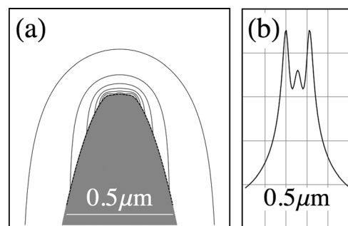
FIG. 9. (a) Plot of the electric field intensity around the tip for three line charges charge. The contour spacing is 10 \text{ MV/m} . (b) Electric field intensity profile along the dashed line in (a). The vertical separation of the grid lines is 20 \text{ MV/m} .
