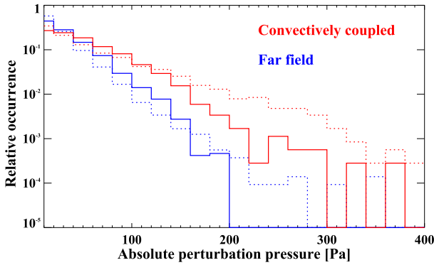
FIG. 11. Simulated absolute perturbation pressure amplitudes in the vicinity of precipitating regions (red), defined as areas separated by less than 0.75° of latitude/longitude from locations where rain rates greater than 1 mm (10 min) -1 are observed and far-field areas (blue). Simulated data are shown as solid histograms and observed data are shown as dashed histograms. All data are normalized by the total number of grid points that lie in the far field and in the vicinity of convection, respectively.
