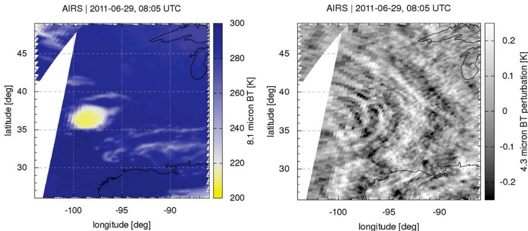
FIG. 12. (left) The 8.1- and (right) 4.3-μm brightness temperature perturbations observed by AIRS at 0805 UTC 29 Jun indicate a mesoscale convective system with convection overshooting the tropopause and eastward-propagating gravity waves, respectively. The images are computed using the method described in Hoffmann and Alexander (2010).
