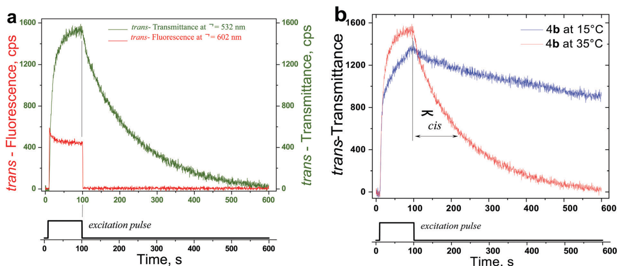
Fig. 4 (a) The temporal evolution of the trans -transmittance (green line) and trans -fluorescence (red line) for the 4b at the sample temperature T = 35 °C. (b) The temperature dependence of the temporal evolution of the trans -transmittance for the 4b compound at T = 15 °C (blue line) and at T = 35 °C (red line); conditions: intensity of the probe beam is constant, 1 \mu\text{W} \times \text{cm}^{-2} , excitation duration \Delta t = 90 s; dye ( 1 \times 10^{-4} M)/concentration of Ba 2+ ions 2 \times 10^{-1} M, pump beam intensity I_{pump} = 4 \text{ mW} \times \text{cm}^{-2} . The vertical black line is a guide for the eye.
