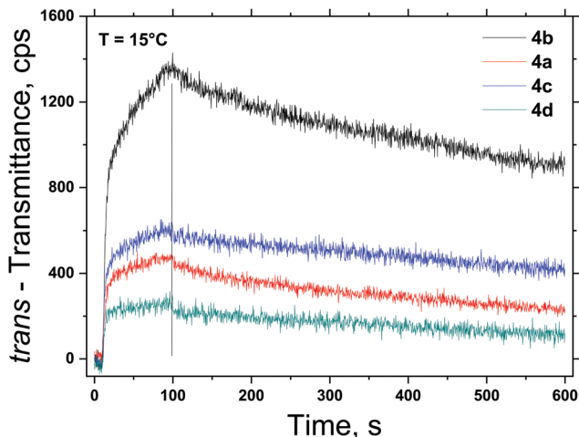
Fig. 5 The temporal evolution of the trans -transmittance for the 4a–4d compounds at a constant temperature of T = 15^\circ\text{C} . Conditions: the intensity of the probe beam is constant, 1\ \mu\text{W} \times \text{cm}^{-2} , excitation duration \Delta t = 90\ \text{s} , dye ( 1 \times 10^{-4}\ \text{M} )/concentration of \text{Ba}^{2+} ions 2 \times 10^{-1}\ \text{M} , pump beam intensity I_{\text{pump}} = 4\ \text{mW} \times \text{cm}^{-2} . The vertical black line is a guide for the eye.
