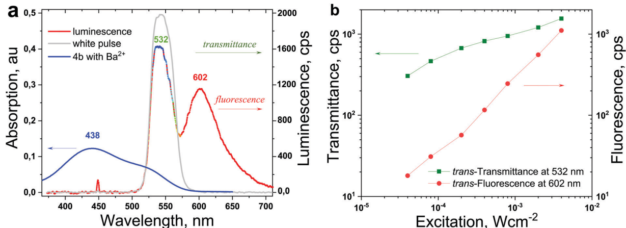
Fig. 3 (a) The optical signal obtained from the trans -dye-Ba 2+ complex excited simultaneously with a pumping beam ( \lambda_{exc} = 450 nm) and a probe beam ( \lambda_{probe} = 532 nm), the continuous wave (cw) registration is the multicoloured line. (b) Dependence of sample transmittance and fluorescence on the intensity of the pump beam; conditions: intensity of the probe beam is constant, 1 \mu\text{W} \times \text{cm}^{-2} , sample temperature T = 22 °C, excitation duration \Delta t = 90 s; 4b ( 1 \times 10^{-4} M)/concentration of Ba 2+ ions, 2 \times 10^{-1} M.
