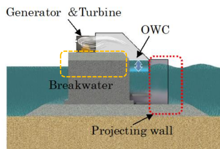
Fig.1 Concept of PW-OWC type wave energy conversion(WEC) breakwater 2.1 Hydraulic model experiments of PW 1),2)
