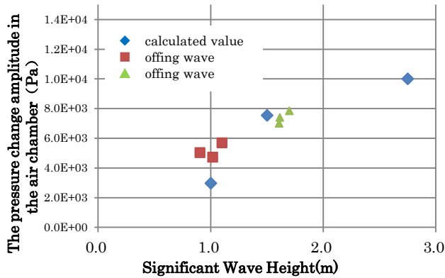
Fig.11 Comparison between observed value and calculated value of the pressure in the air chamber
