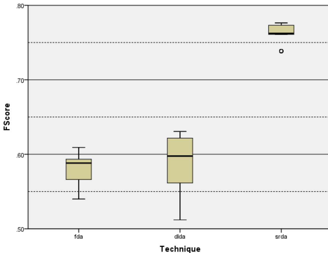
Fig. 23. Boxplot of F-Scores for Discriminant Analysis Methods.
