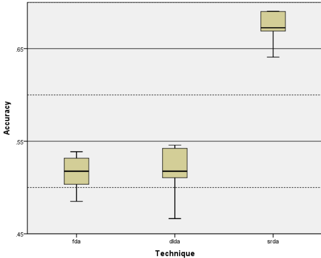
Fig. 22. Boxplot of Accuracies for Discriminant Analysis Methods.
