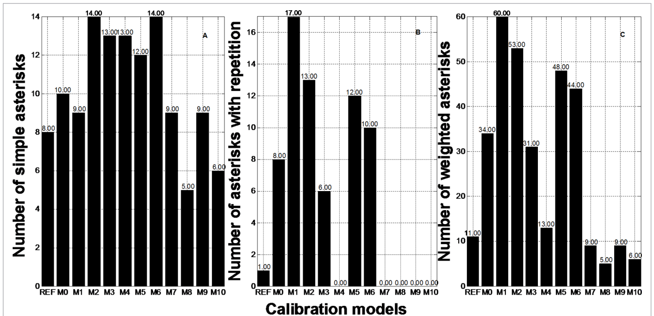
Figure 4. Bar graphs of the penalties for each calibration model submitted in the interlaboratory programme of 2013: (A) number of simple asterisks, (B) number of asterisks with repetition and (C) number of weighted asterisks.
