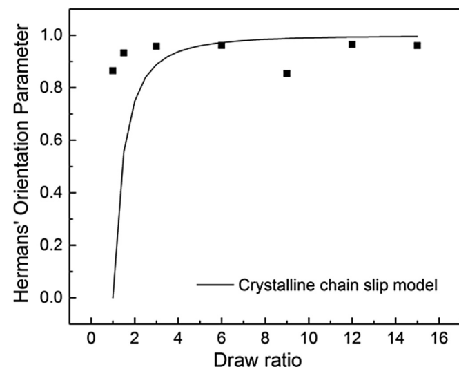
Fig. 7. Hermans' orientation parameter values as a function of draw ratio. The solid line represents the crystalline chain slip model according to Equation (4).
