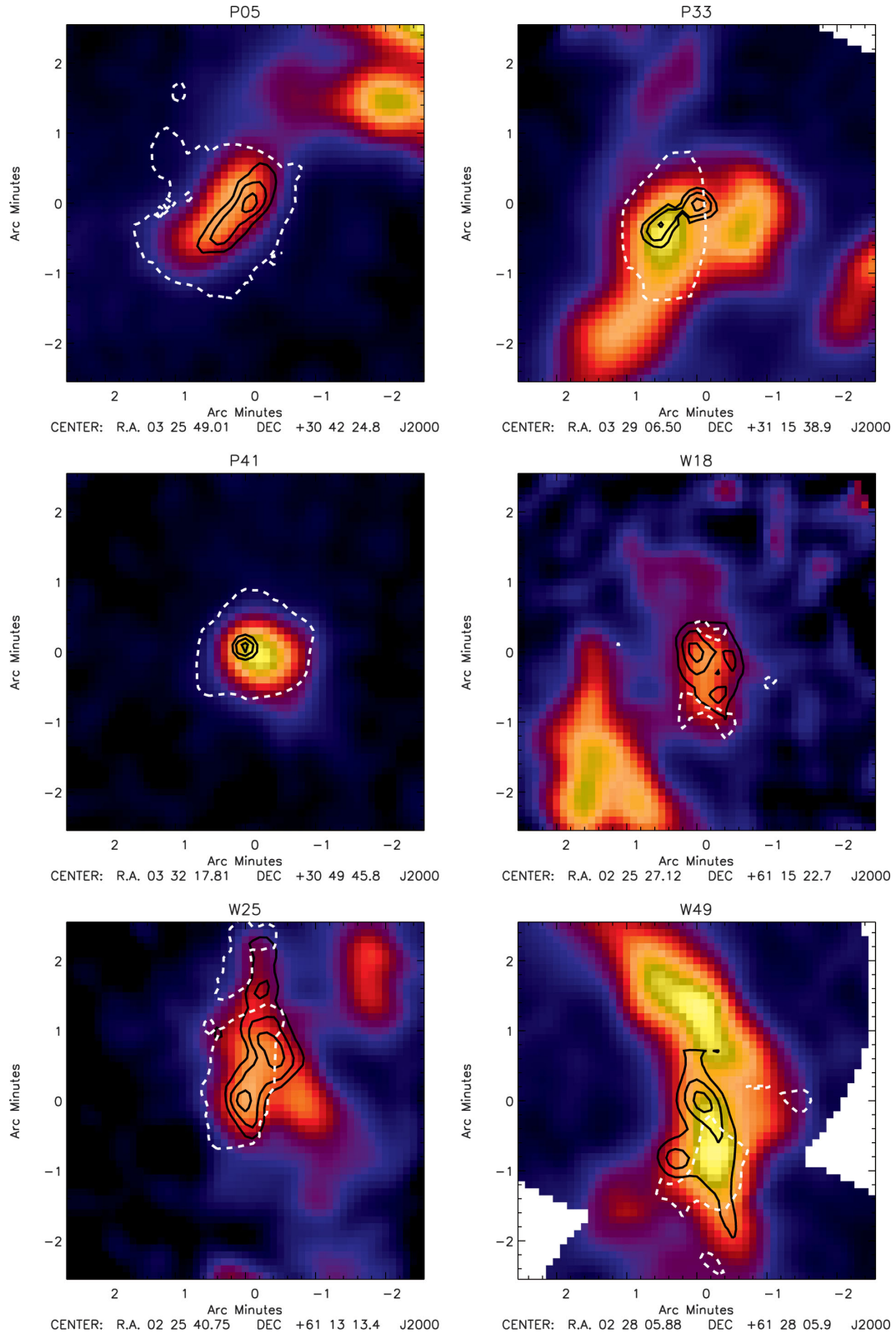
Figure 11. \text{NH}_3 integrated intensity in sources P05, P33 & P41 and W18, W25 & W49, overlaid with black contours of submillimetre emission at 50, 70 and 90 per cent of the peak flux density. A white, broken contour traces the \text{NH}_3 column density distribution at a level of 50 per cent of the local peak for all sources except W18, for which the contour level is 40 per cent. The full set of figures is available online.
